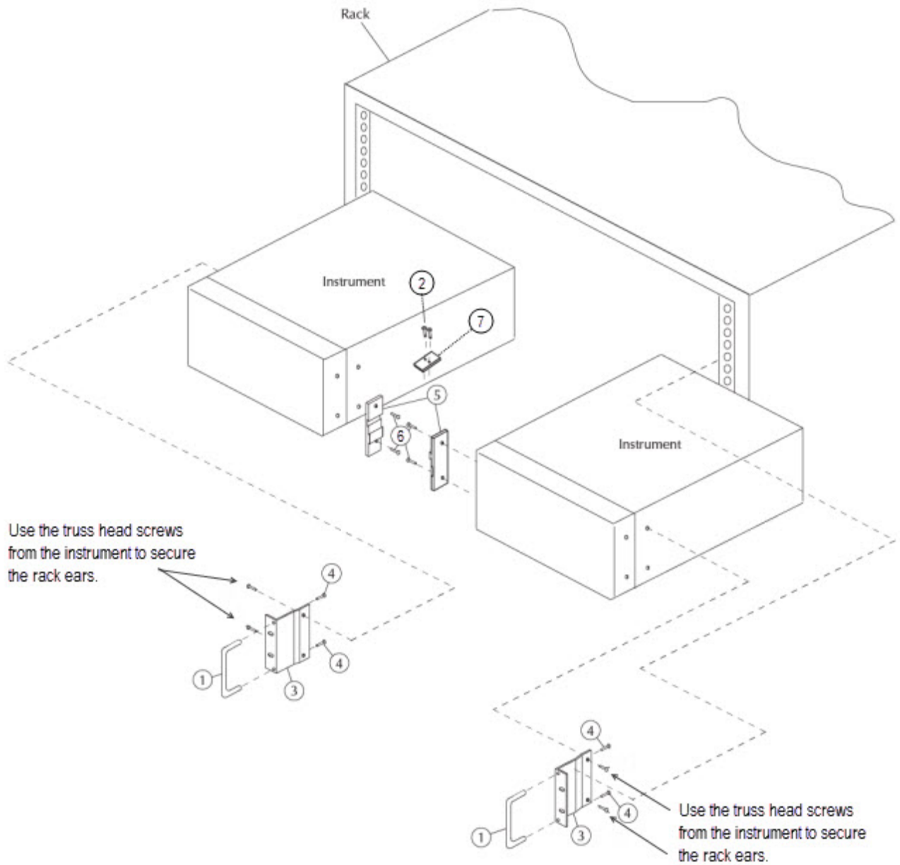
Figure 1: Model 2290-5 double rack mount kit installation
