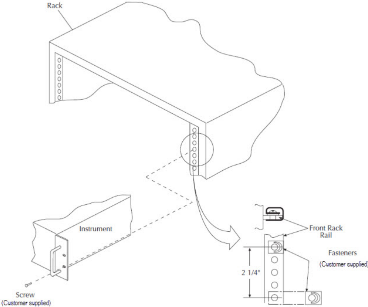
Figure 2: Model 2290-5 suggested rack fastener installation
