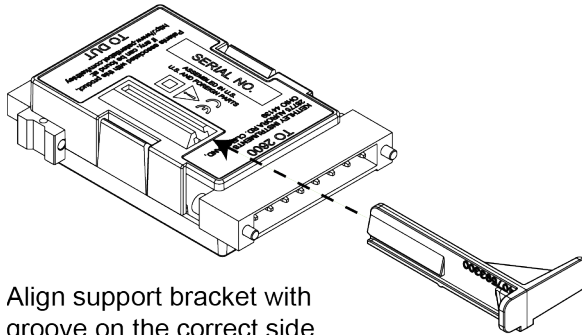
Figure 3: Installing the support bracket for use in channel A
