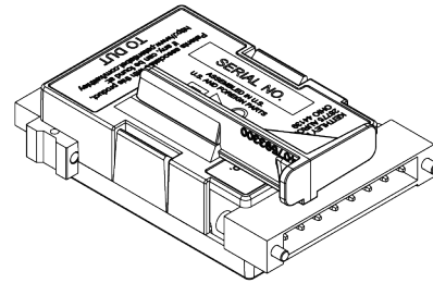
Figure 3: Installing the support bracket for use in channel A
