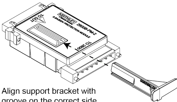
Figure 4: Installing the support bracket for use in channel B
