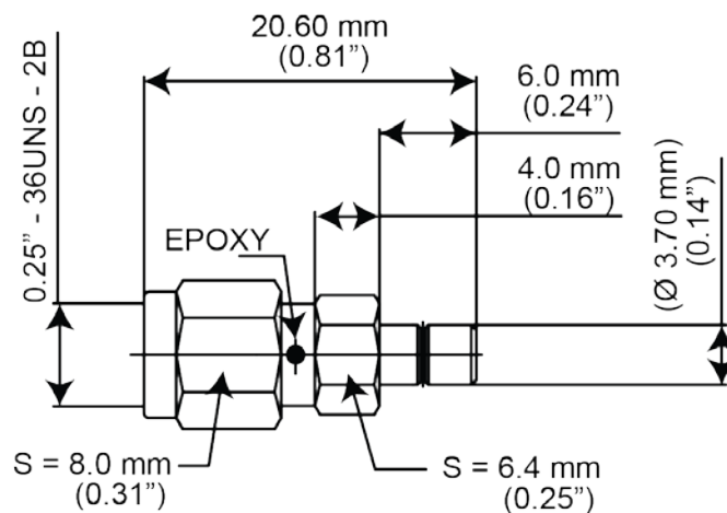
Figure 2: SMA (M) to SMB (M) adapter connector saver dimensions
