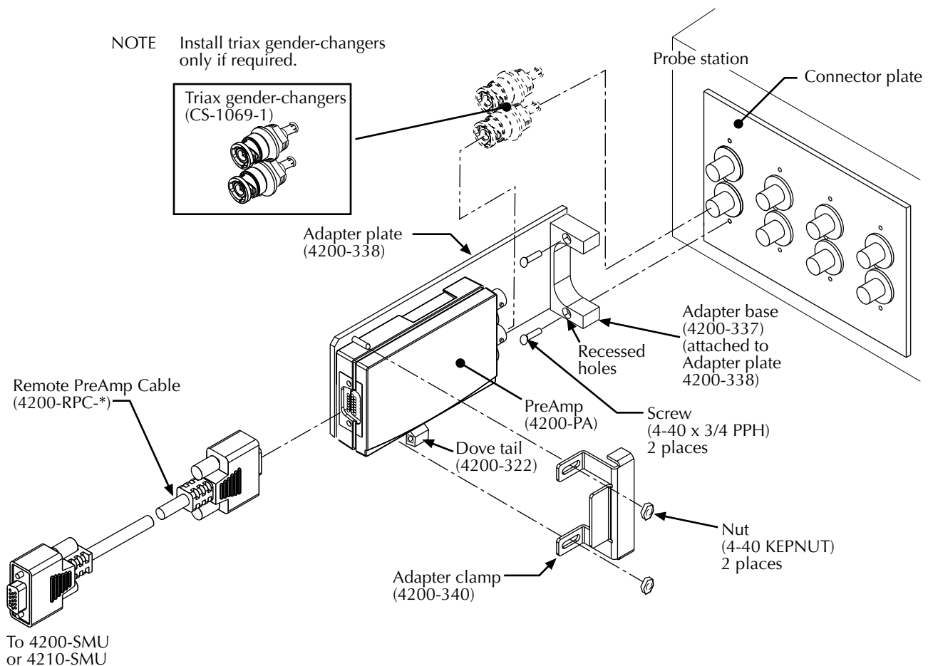
Figure 2 Adapter assembly
