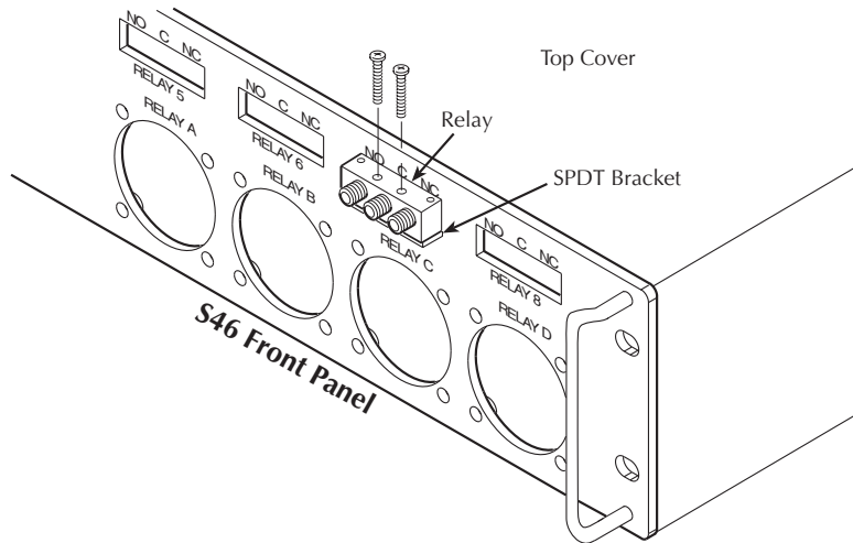
Figure 1 RELAY 1-8 installation
