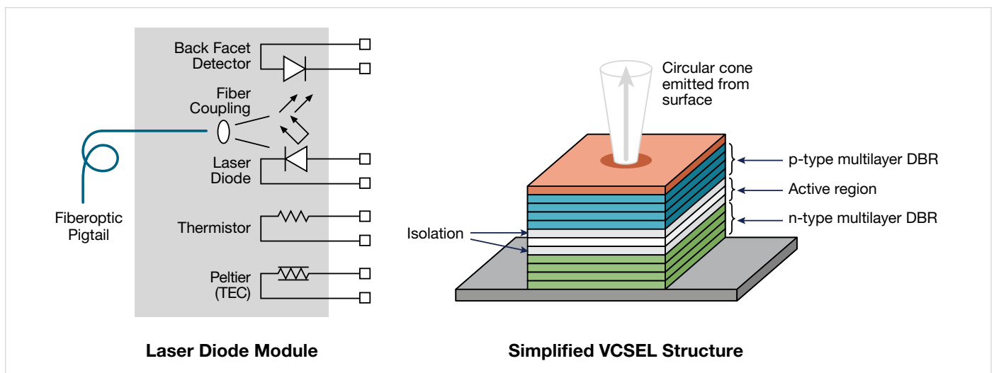
Figure 1. A simplified VCSEL structure.
