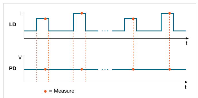
Figure 15. Pulse I-V sweep.
