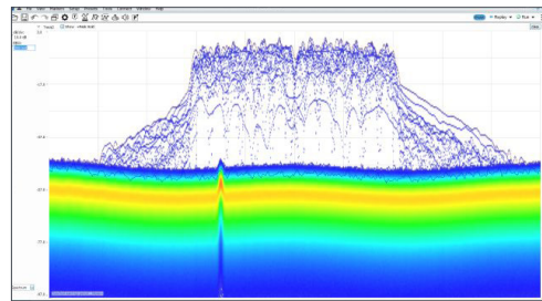
See lower power in band signals with DPX Spectrograms.
