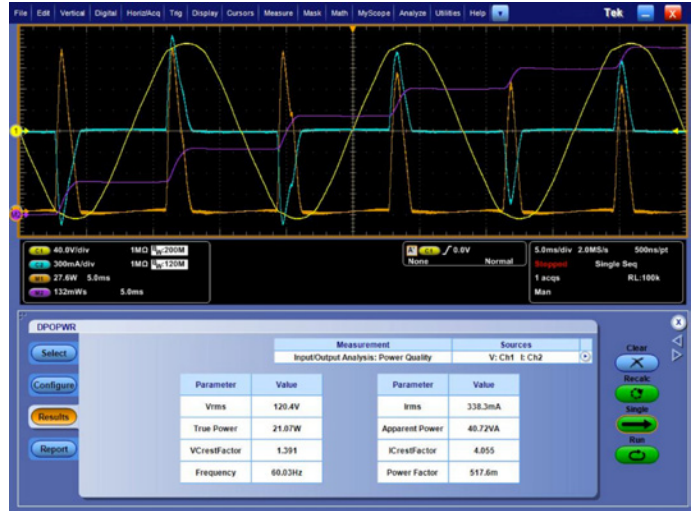
Figure 11. Power Quality Measurements on a PC power adapter after the laptop battery is charged while the laptop is running.
