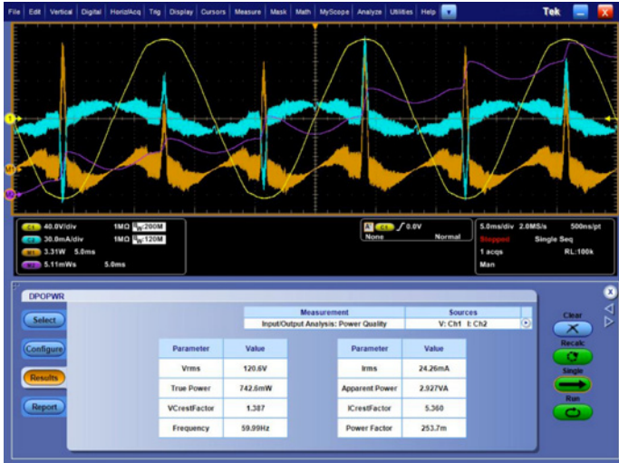
Figure 12. Power Quality Measurements on a PC power adapter after the laptop battery is charged, with the laptop turned off.
