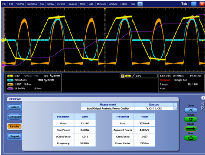
Figure 8. Voltage, Current, Power, and Energy Readouts.
