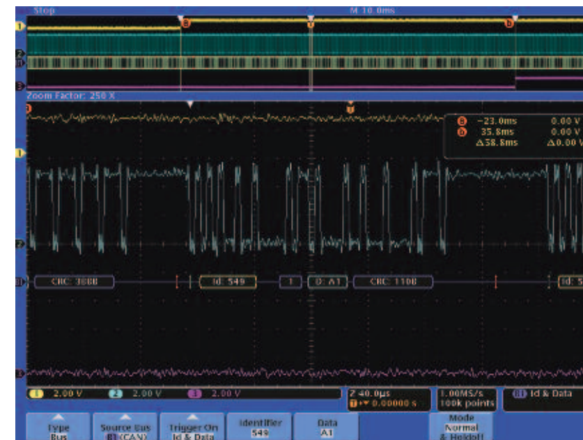
Automatically decode serial bus information in correlation to the live signal in an easy to read format
