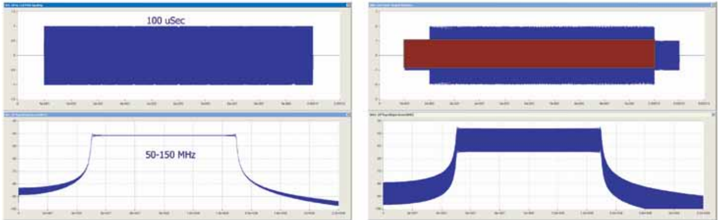
Figure 6. Transmitted LFM signal (left) versus returned signal with 2 targets (right): the brown area in the time domain view is where the target returns overlap.
