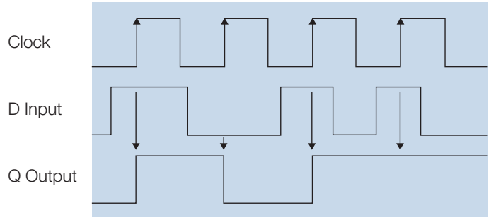
Figure 15. 74F74 D-Flip-Flop.
