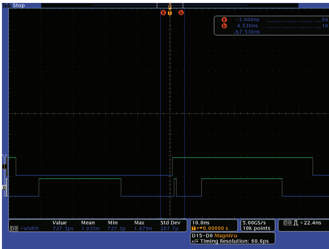
Figure 13. Triggering on 727.3 ps glitch on the bottom LVPECL signal.
