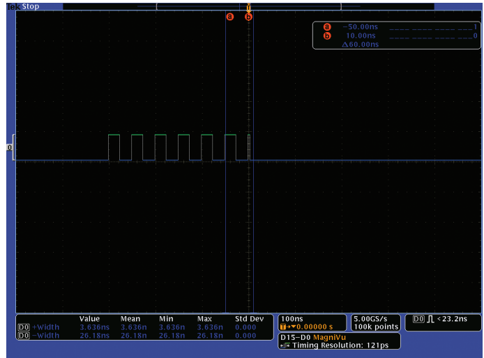
Figure 11. Triggering on positive pulse width error of 3.636 ns.
