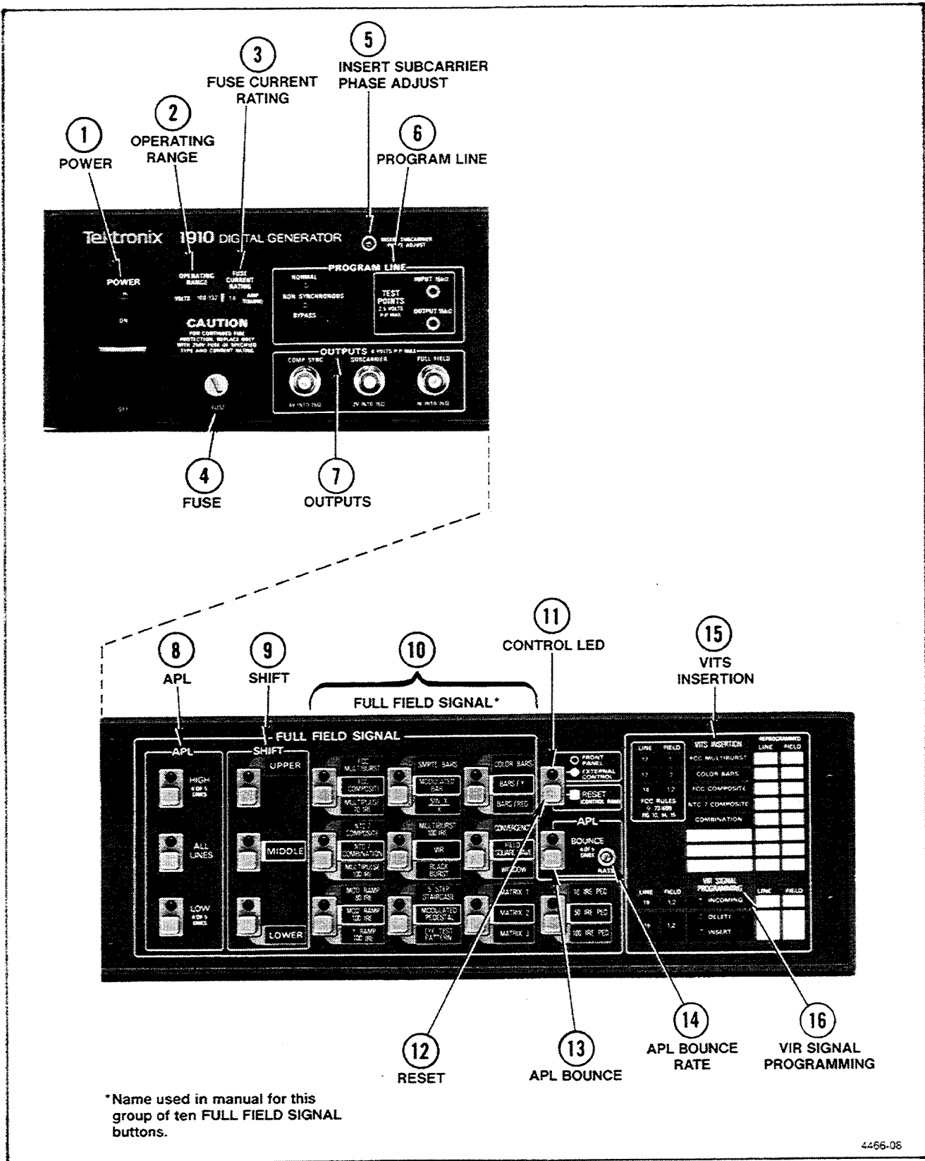
Fig. 3-1. 1910 Front Panel.
