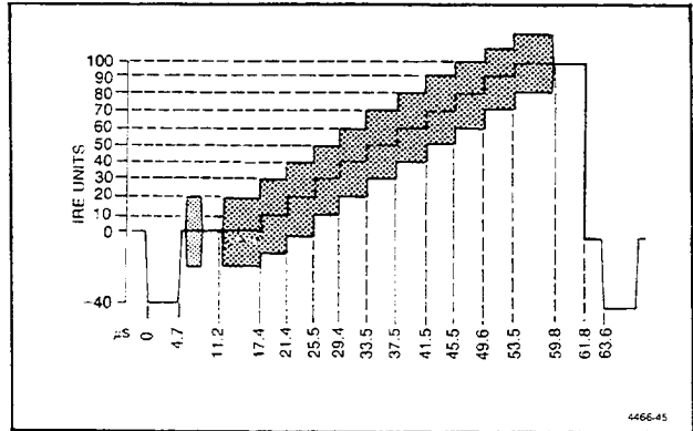
Fig. 6-20. Modulated 10-Step.
