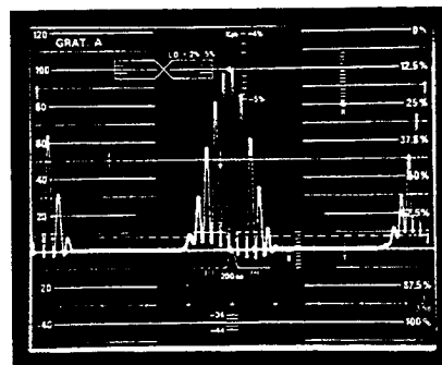
Figure 4 (c) 3.58 MHz
