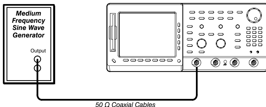
Figure 1-18: Initial Test Hookup—TDS 520A or 524A Only
