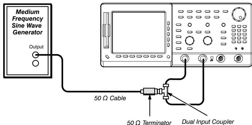
Figure 1-10: Initial Test Hookup
