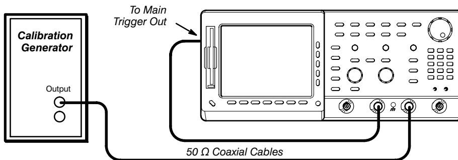
Figure 1-21: Initial Test Hookup
