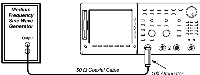
Figure 1-14: Initial Test Hookup
