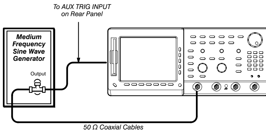
Figure 1-19: Initial Test Hookup—TDS 540A or 544A Only
