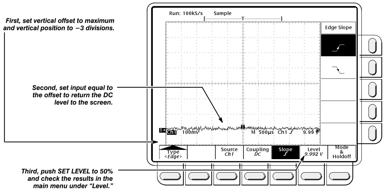
Figure 1-17: Measurement of Trigger-level Accuracy
