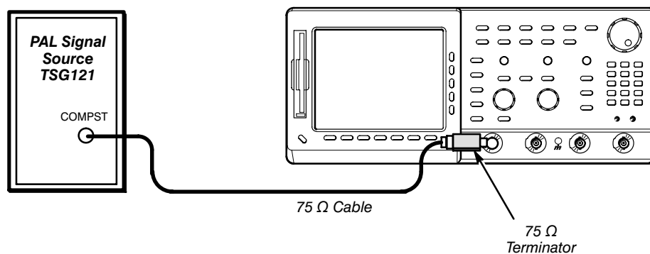
Figure 1-36: Line Count Accuracy Test Hookup
