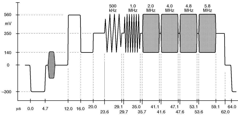
Figure 1-14: PAL Multiburst
