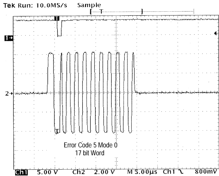
Figure 455-17: 17 bit Word
