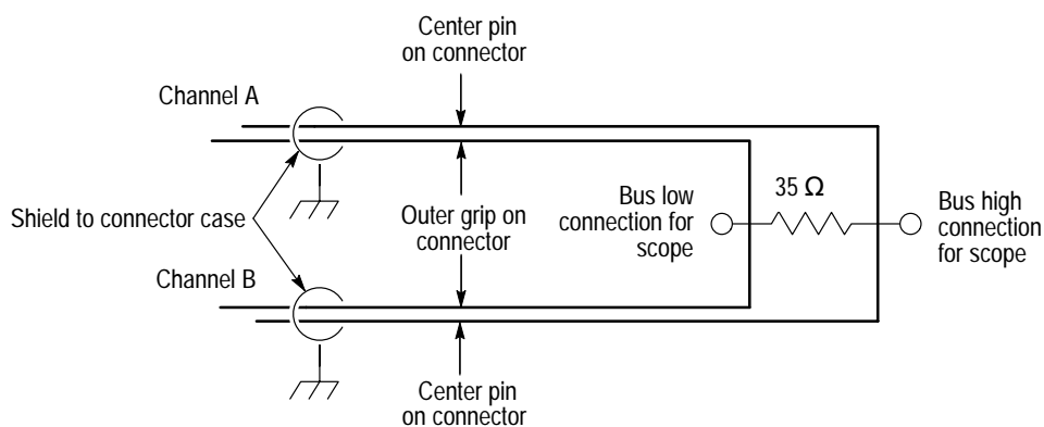
Figure 455-7: Cable Diagram
