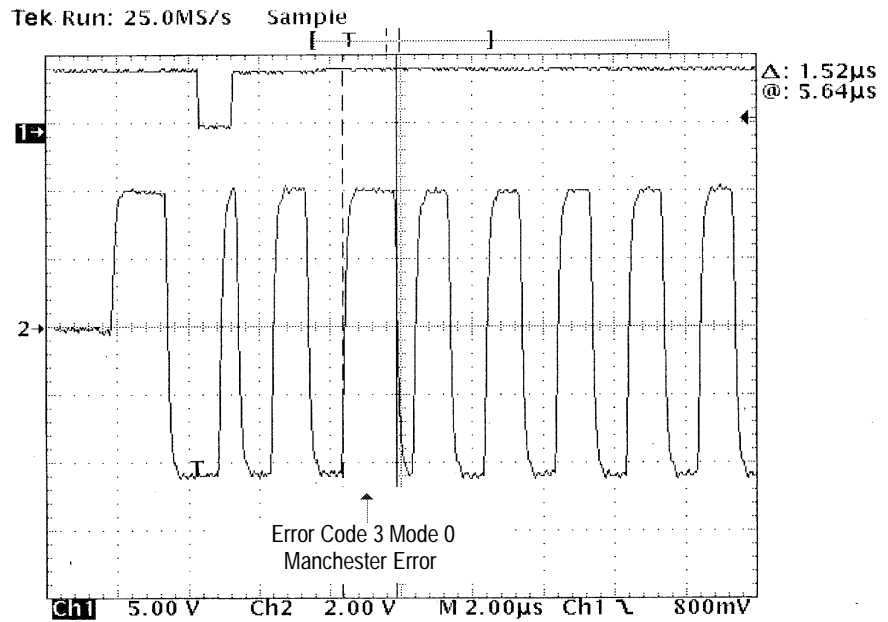
Figure 455-15: Manchester Error.
