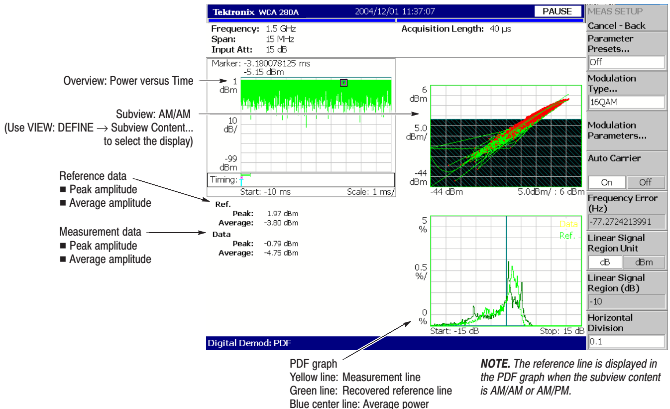
Figure 3–50: PDF measurement
