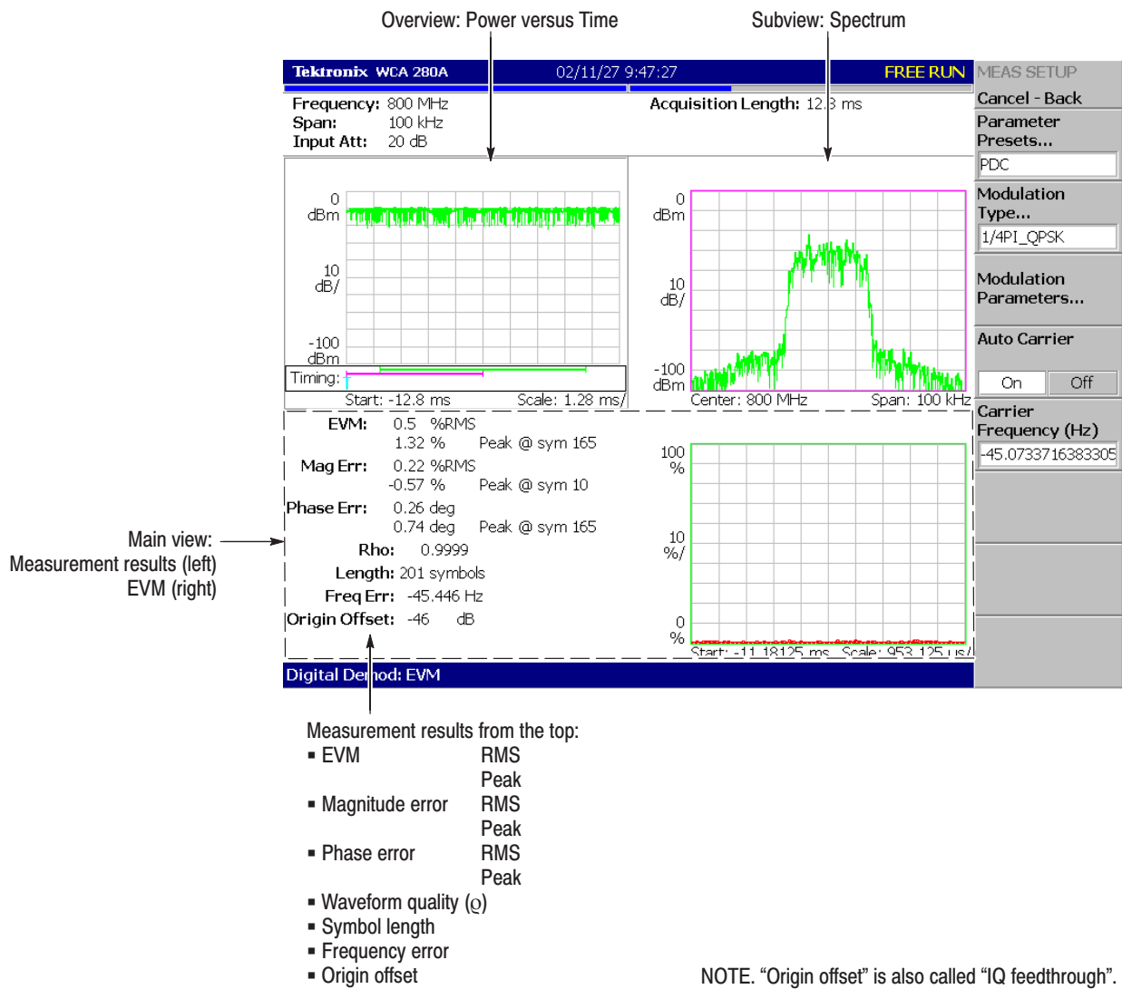
Figure 3–41: EVM measurement
