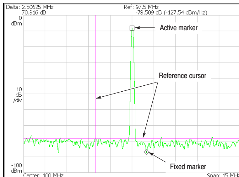
Figure 3-150: Marker display
