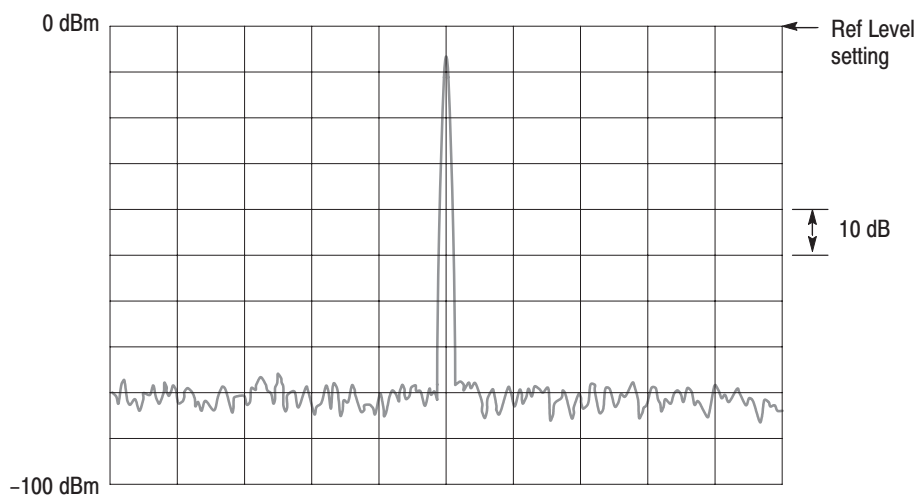
Figure 2–35: Setting amplitude
