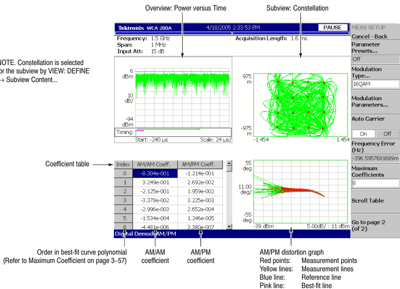
Figure 3–48: AM/PM measurement
