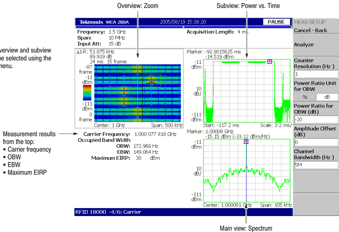
Figure 3–52: Carrier measurement
