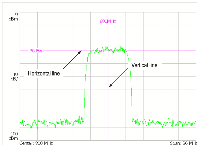
Figure 3–144: Display line
