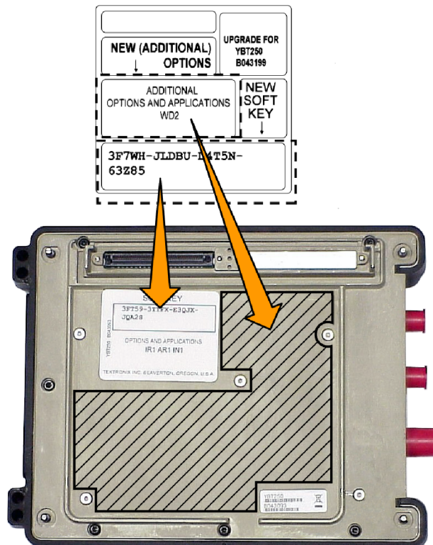
Figure 1: YBT250 new label positions.
