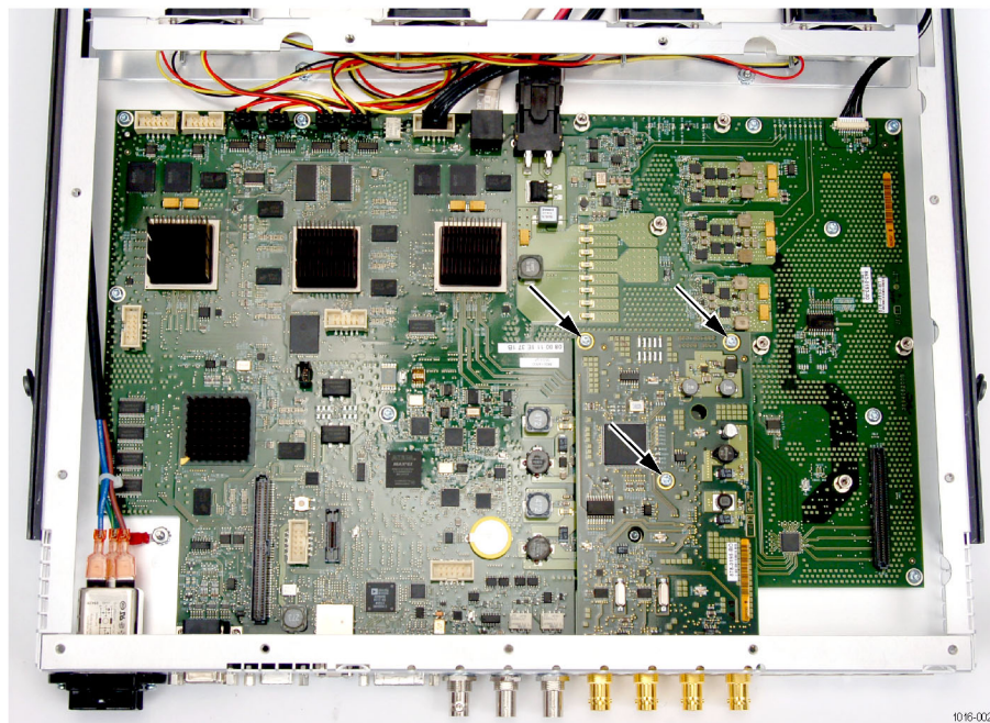
Figure 3: SDI board
