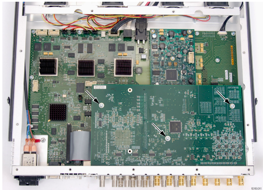
Figure 19: Audio board installed
