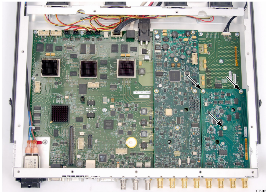
Figure 12: CPS board installation
