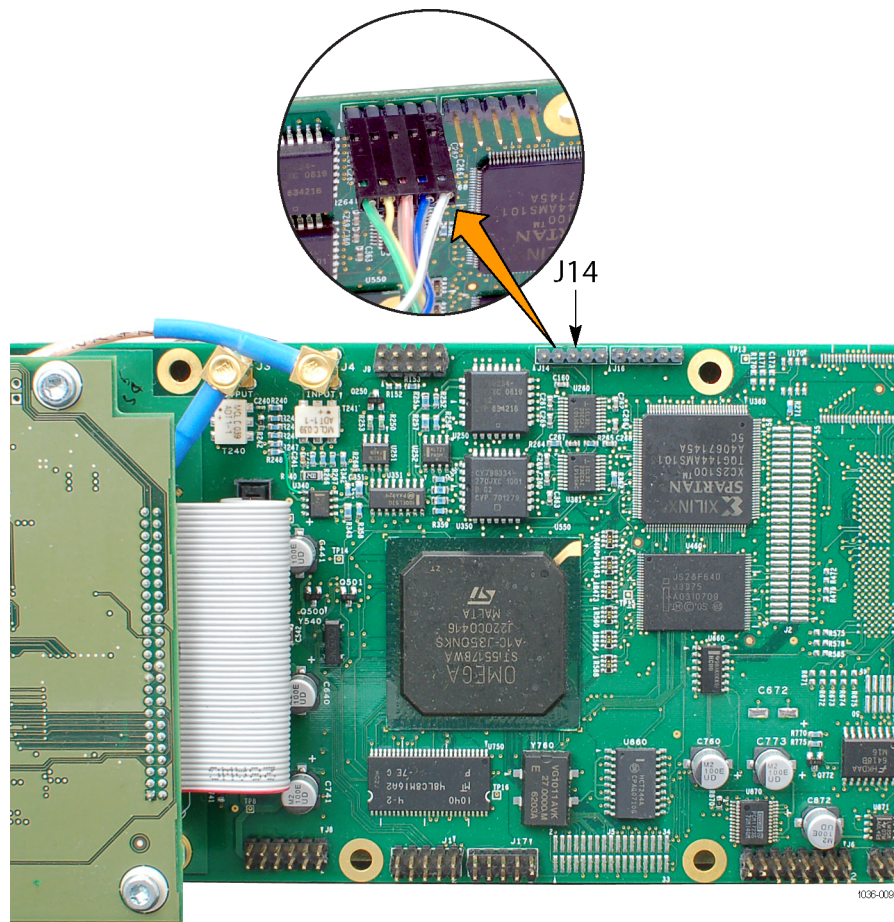
Figure 6: CIP cable installation on option QB2, S2, and VS interface cards
