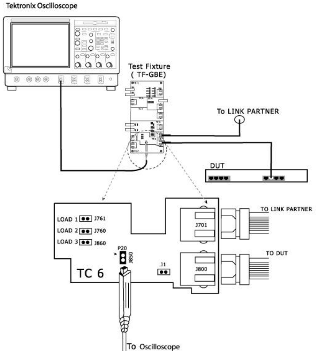
Figure 6-27: 10BASE-T Connections for Jitter without cable
