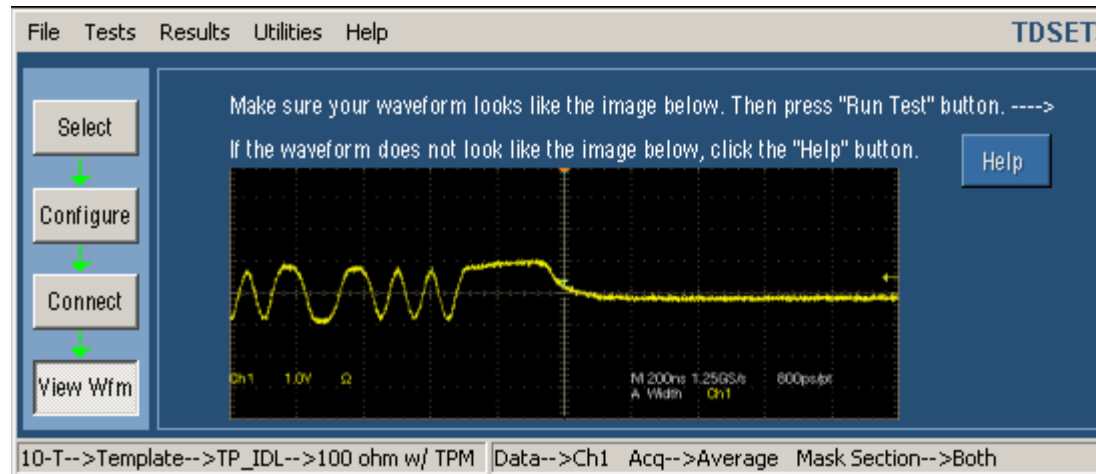
Figure 13-3: 10BASE-T View Waveform for TP_IDL with TPM
