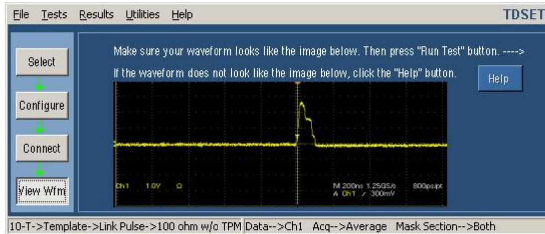
Figure 13-1: 10BASE-T View Waveform for Link Pulse
