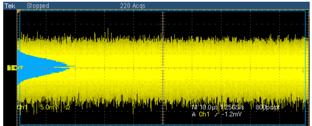
Figure 8-24: Waveform for 1000BASE-T CM Voltage
