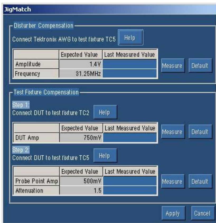
Figure 3-26: Jig Match dialog box for 1000-T Template/Peak Volt/Droop test
