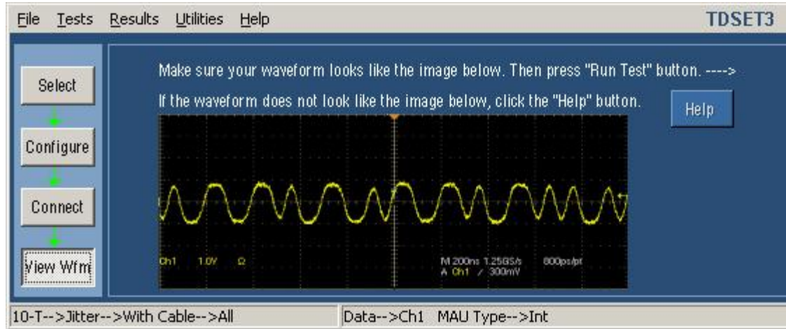
Figure 13-5: 10BASE-T View Waveform for Jitter with cable
