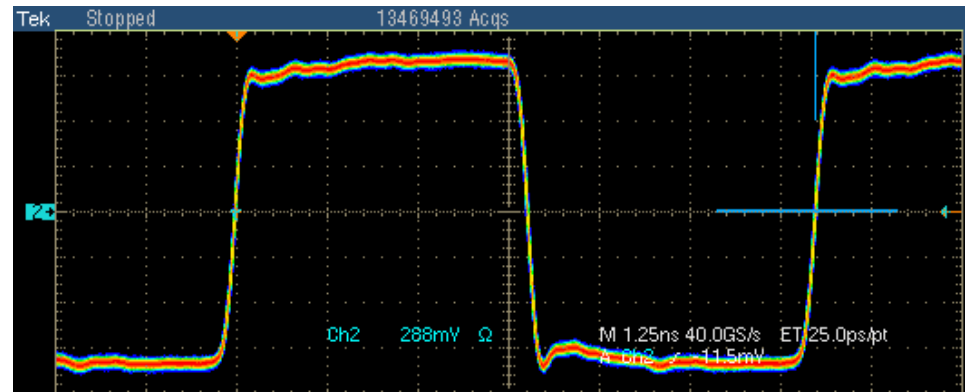
Figure 8-10: Histogram Waveform for 1000BASE-T Jitter Master Unfiltered
