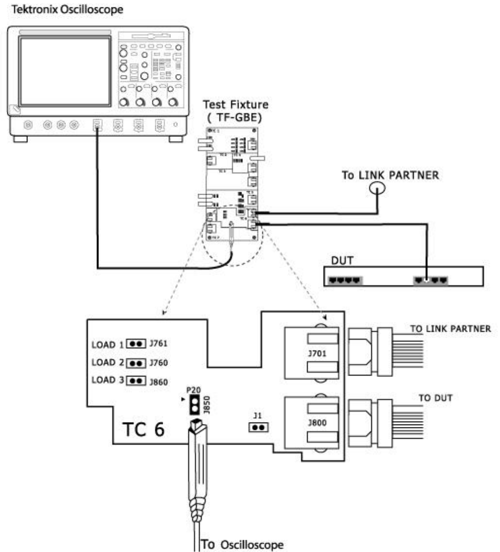
Figure 6-28: 10BASE-T Connections for Differential Voltage
