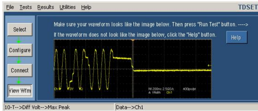
Figure 13-7: 10BASE-T View Waveform for Differential Voltage
