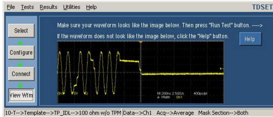
Figure 13-4: 10BASE-T View Waveform for TP_IDL without TPM
