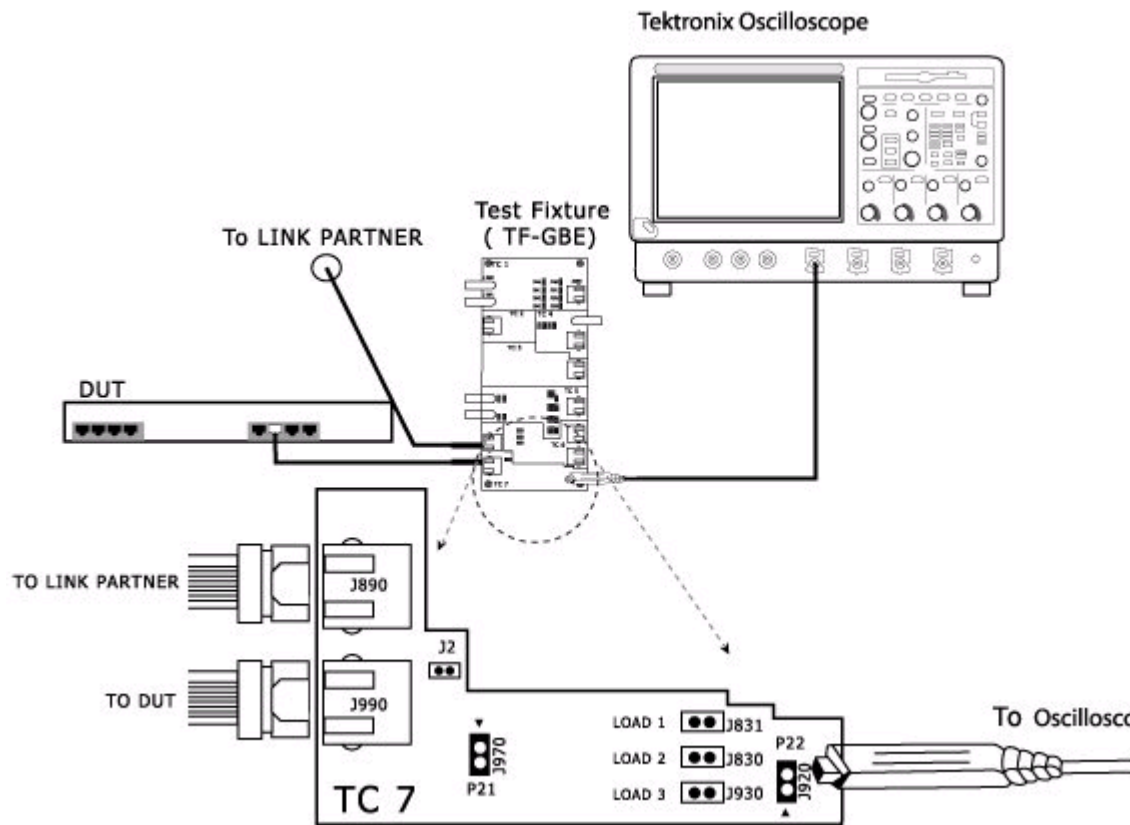
Figure 6-24: 10BASE-T Connections for TP_IDL with Twisted-pair model
