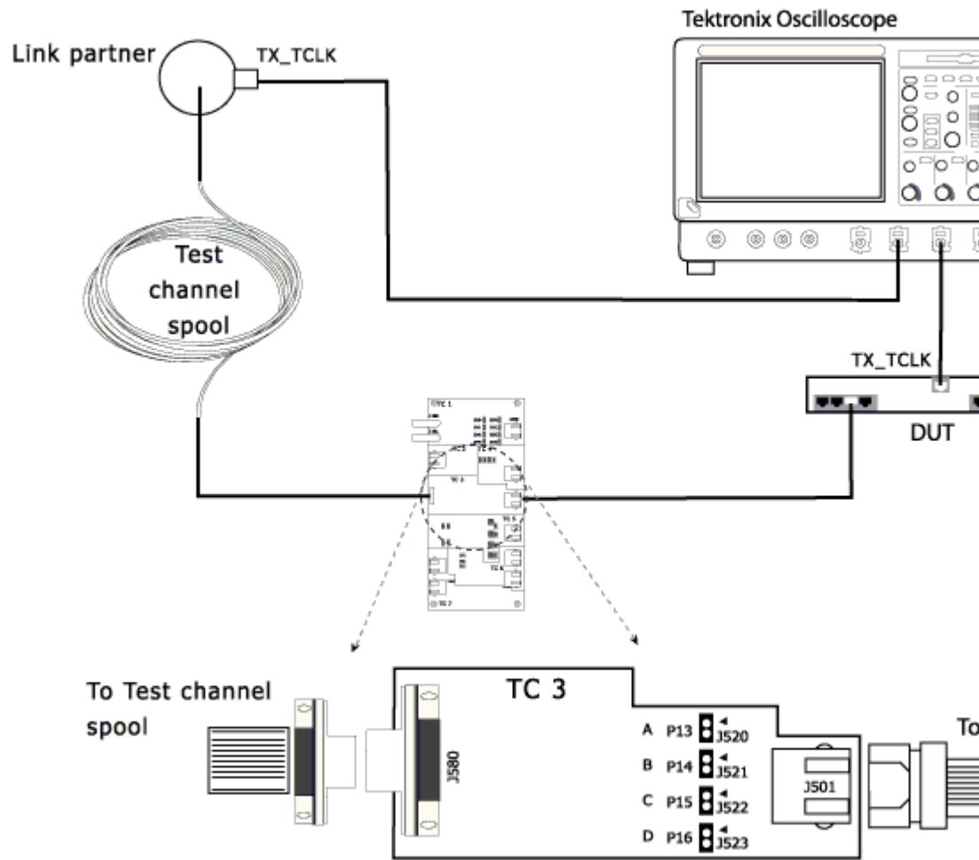
Figure 6-8: 1000BASE-T Step 1 Connections for Jitter Slave Filtered
