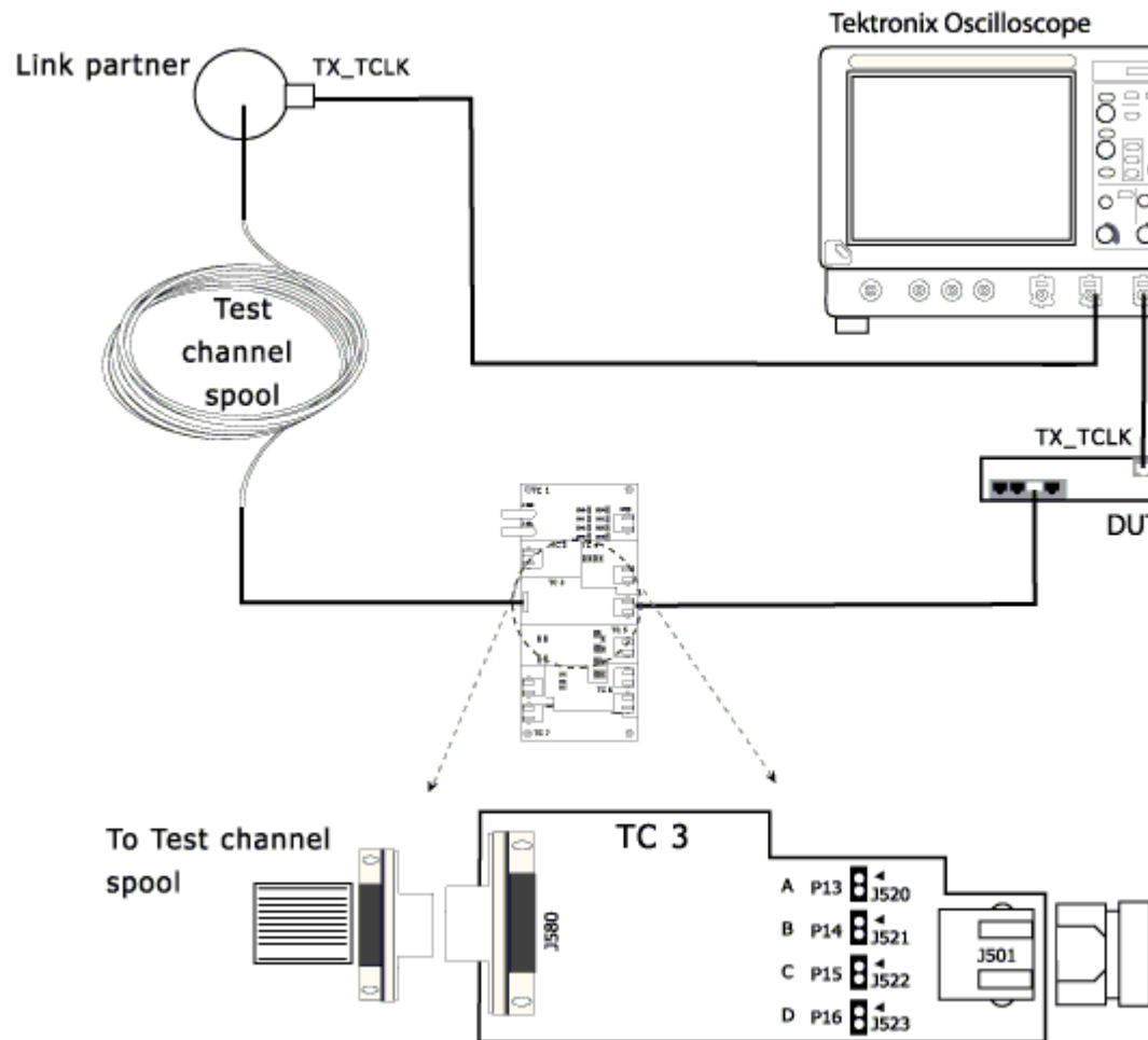
Figure 6-11: 1000BASE-T Connections for Jitter Slave Unfiltered
