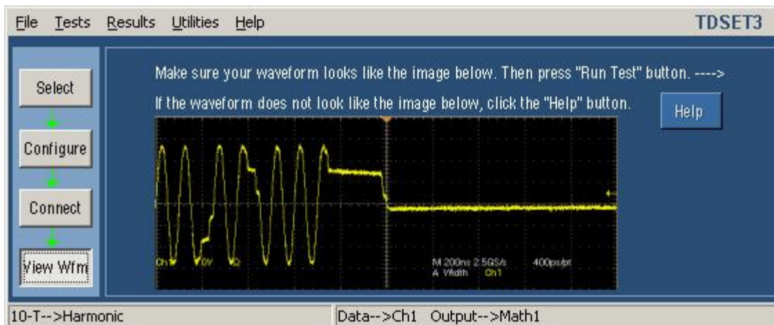
Figure 13-8: 10BASE-T View Waveform for Harmonic
