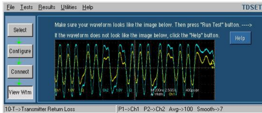
Figure 13-9: 10BASE-T View Waveform for Return Loss
