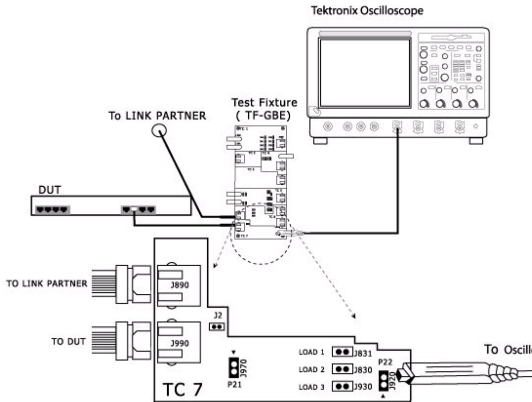
Figure 6-21: 10BASE-T Connections for MAU
