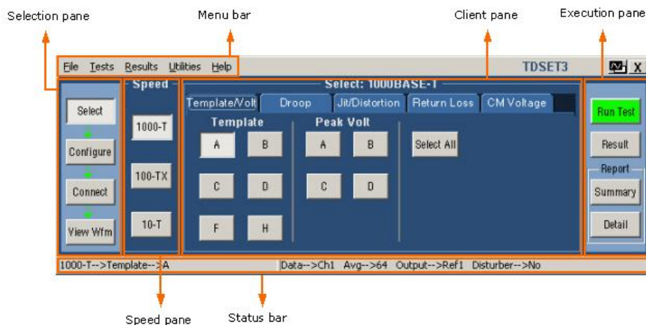
Figure 3-1: Application window
