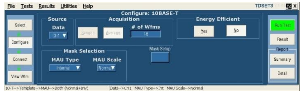
Figure 5-3: 10BASE-T/10BASE-Te Configure pane
