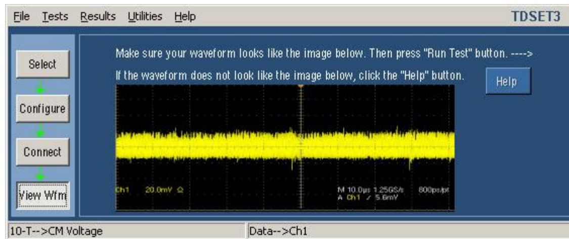
Figure 13-10: 10BASE-T View Waveform for CM Voltage
