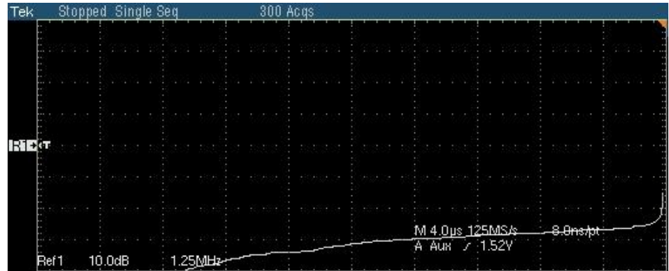
Figure 18-21: Waveform of 10BASE-T Return Loss Load calibration
