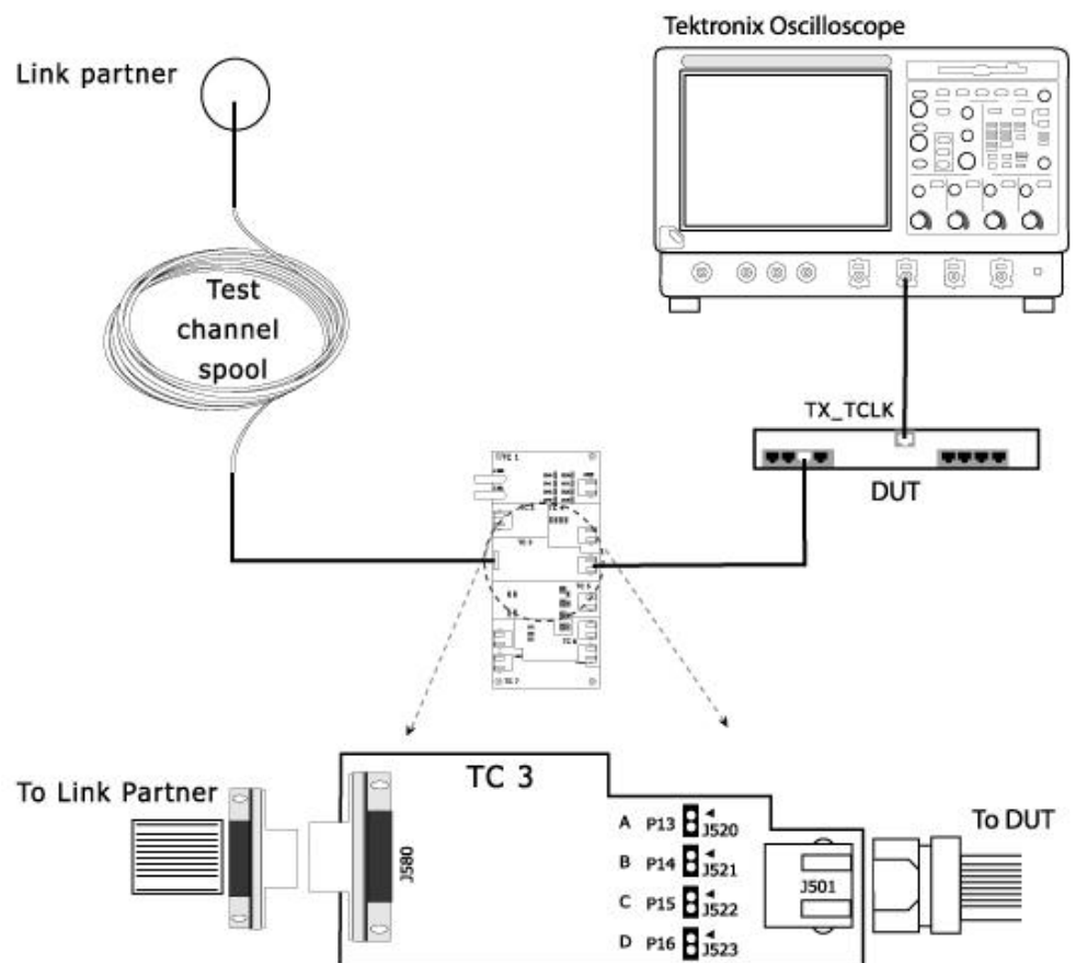
Figure 6-6: 1000BASE-T Connections for Jitter Master Unfiltered
