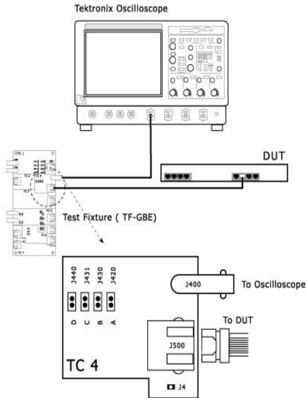
Figure 6-32: 10BASE-T Connections for CM Voltage
