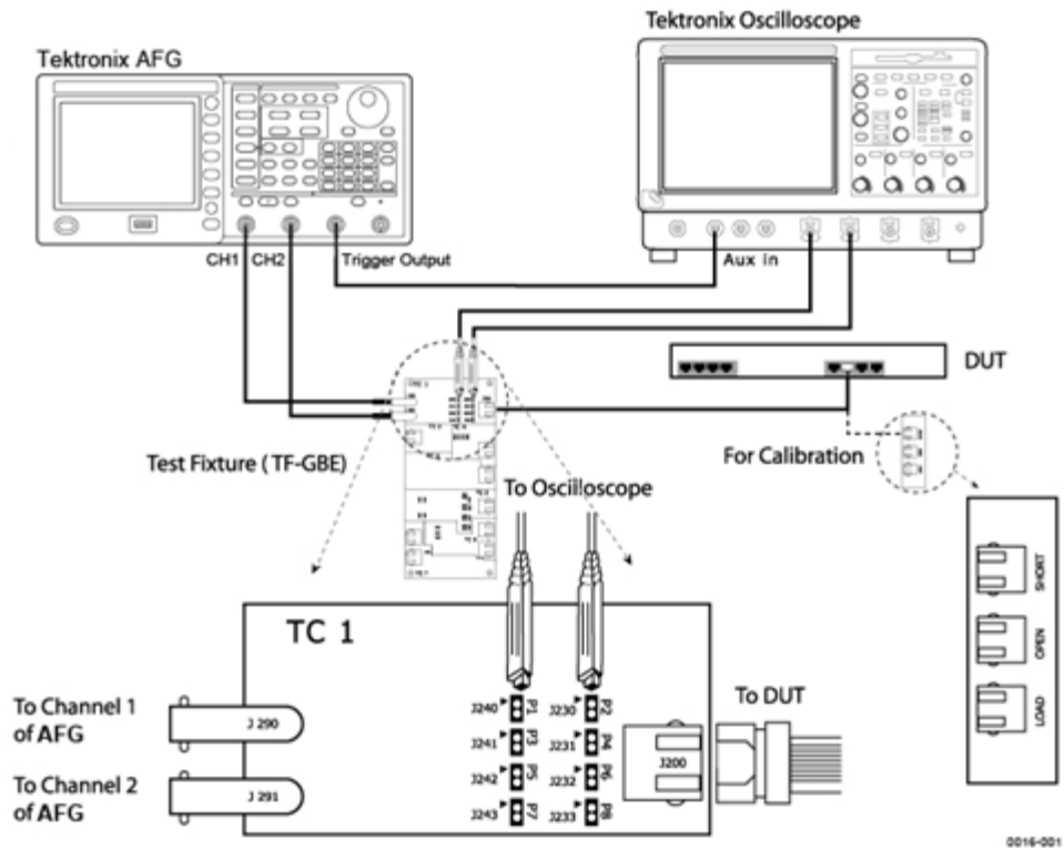
Figure 6-14: 1000BASE-T Return Loss setup using an Arbitrary Function Generator
