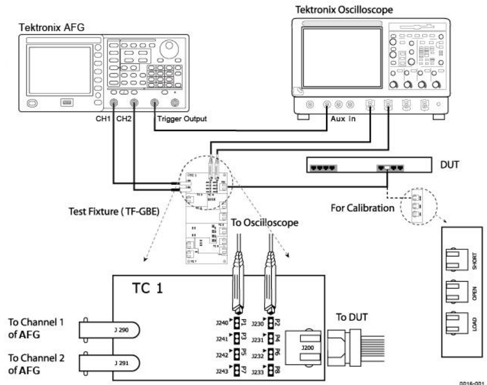
Figure 6-31: 10BASE-T Return Loss setup using an Arbitrary Function Generator
