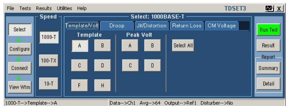
Figure 2-2: Application interface
