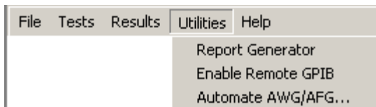
Figure 3-5: Utilities menu
