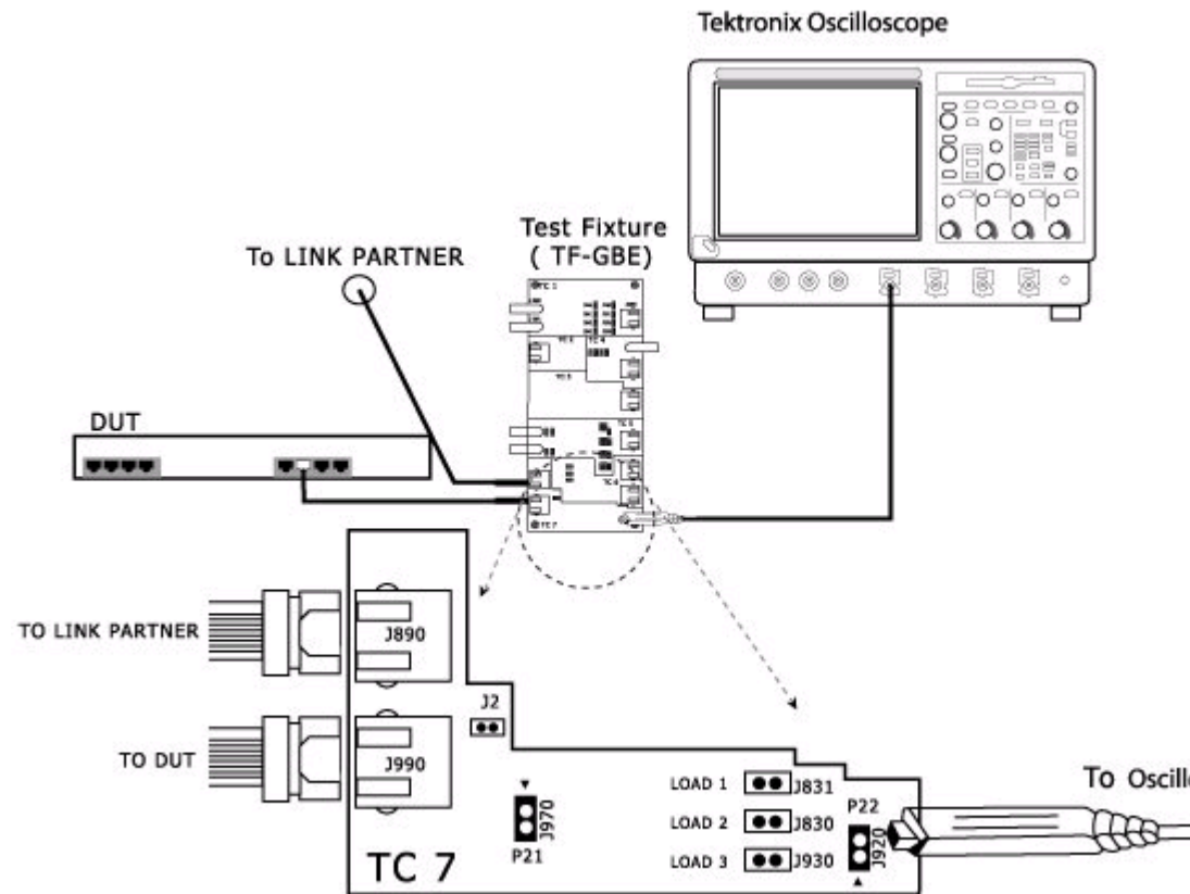
Figure 6-26: 10BASE-T Connections for Jitter with cable
