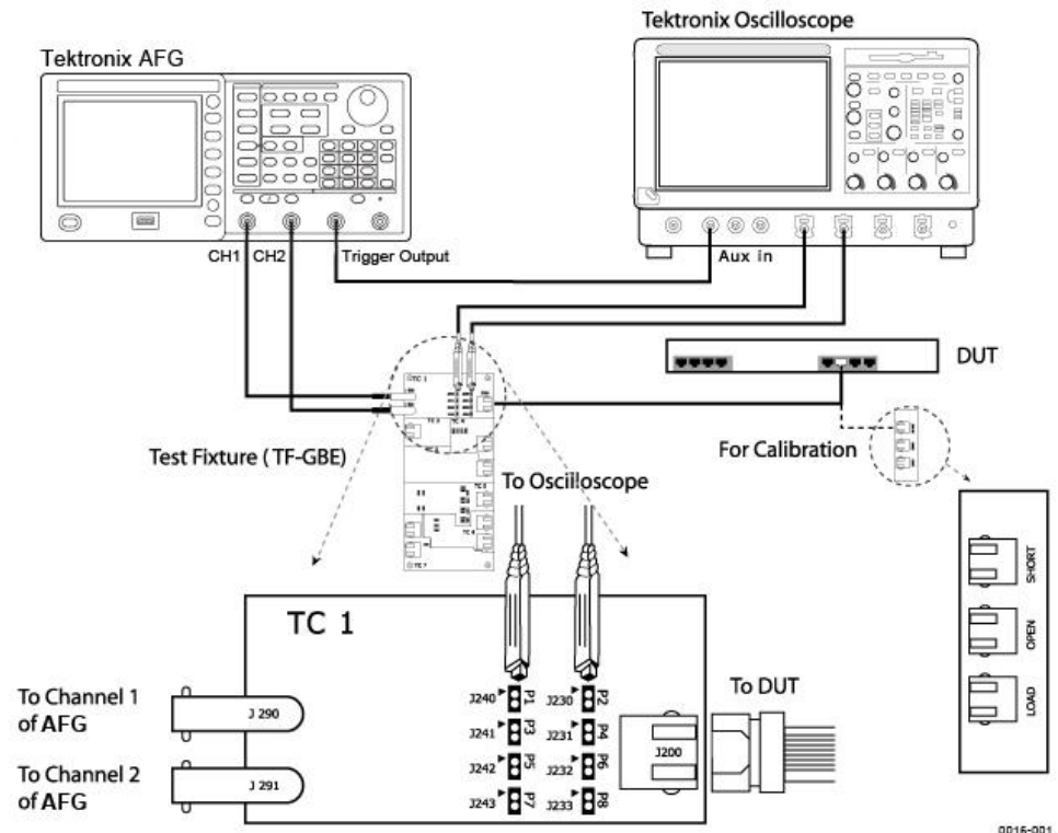
Figure 6-18: 100BASE-TX Return Loss setup using Arbitrary Function Generator
