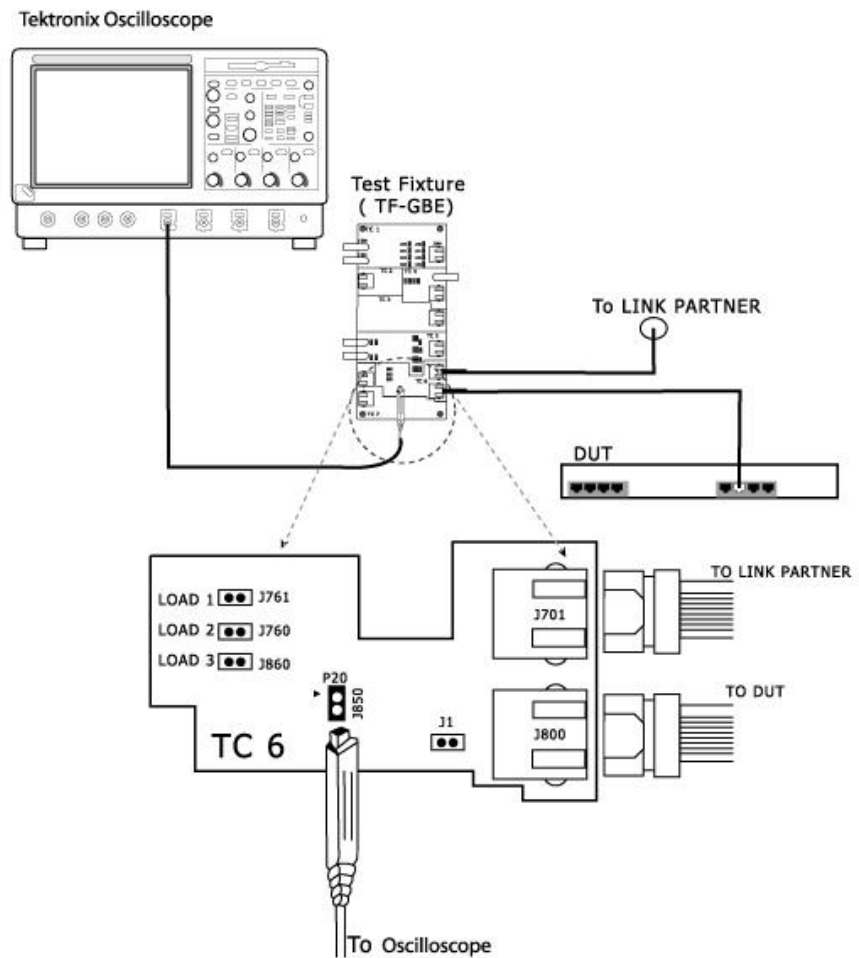
Figure 6-29: 10BASE-T Connections for Harmonic
