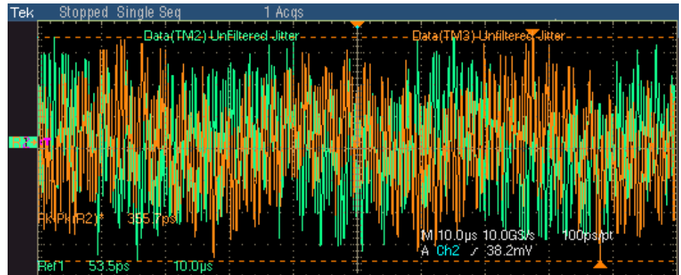
Figure 8-19: TIE Waveform for 1000BASE-T Jitter Slave Unfiltered
