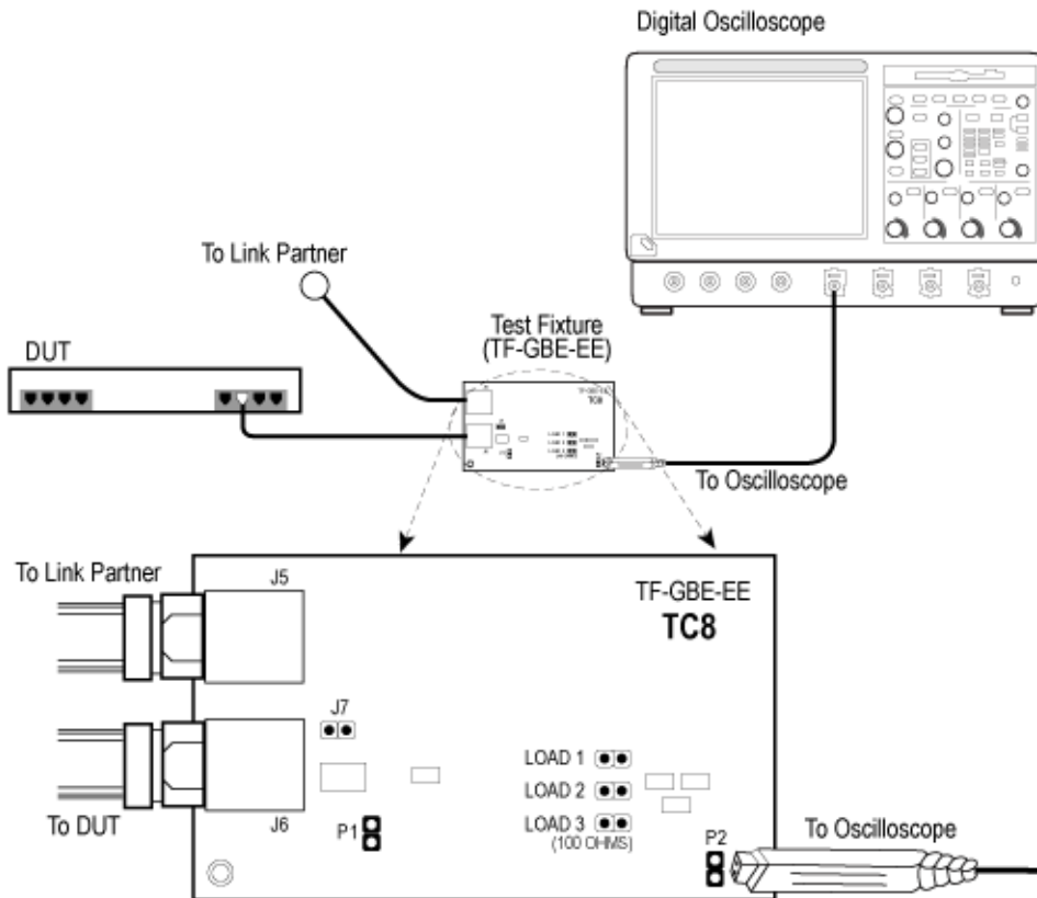
Figure 6-22: 10BASE-T e Connections for MAU
