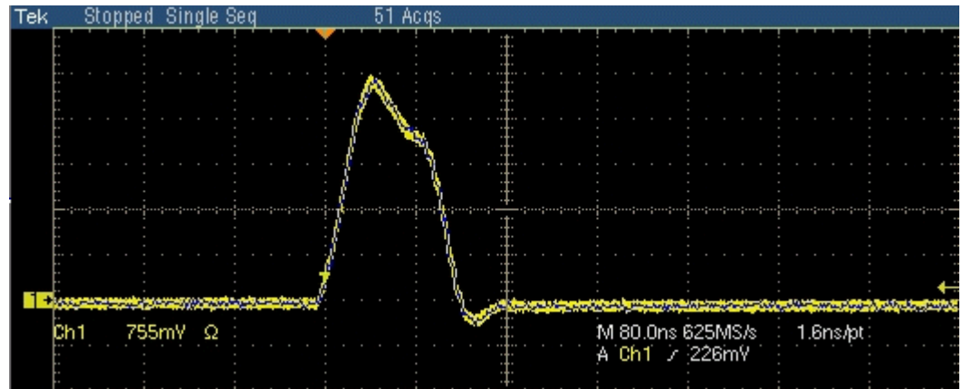
Figure 10-7: Waveform for 10BASE-T Link Pulse timing
