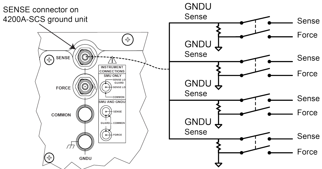
Figure 20: 4200A-CVIV GNDU switching configuration
