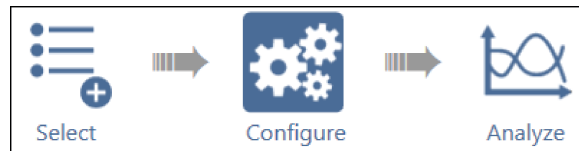
Figure 35: Configure selected
