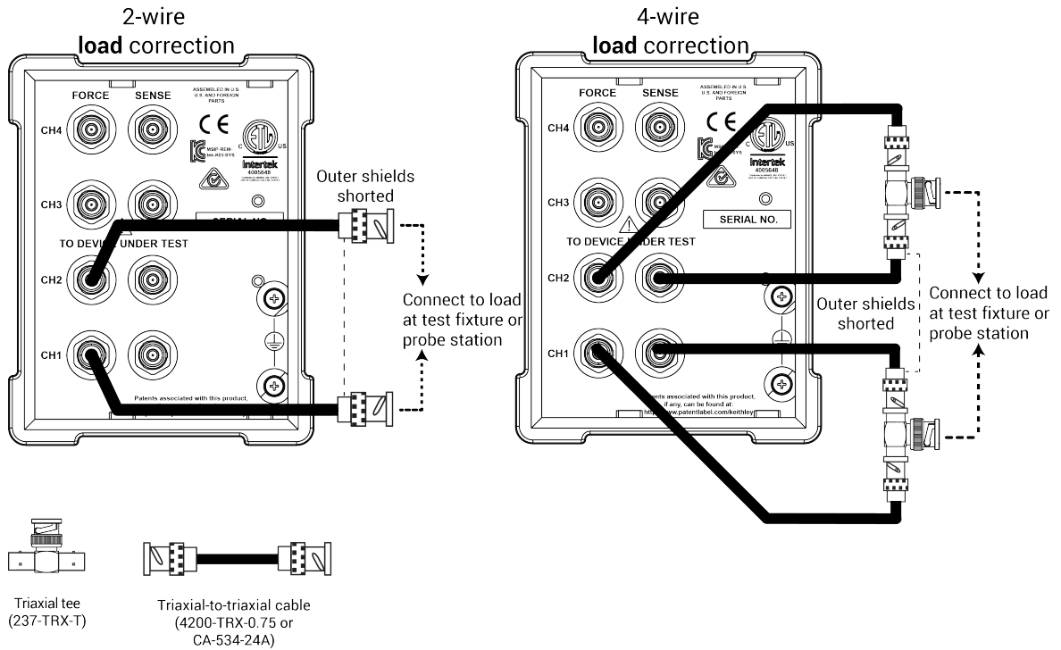
Figure 30: Connections for load connection compensation
