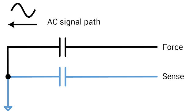
Figure 21: 4200A-CVIV AC coupled AC ground configuration
