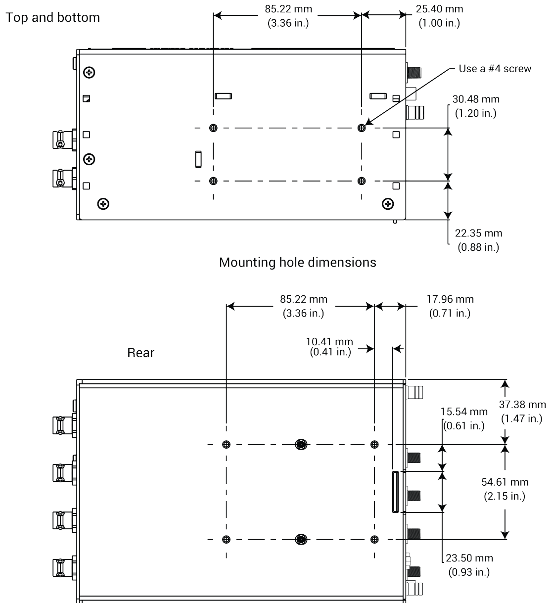
Figure 14: 4200A-CVIV mounting dimensions
