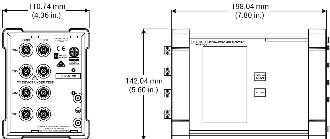
Figure 6: 4200A-CVIV mechanical dimensions, bumpers installed
