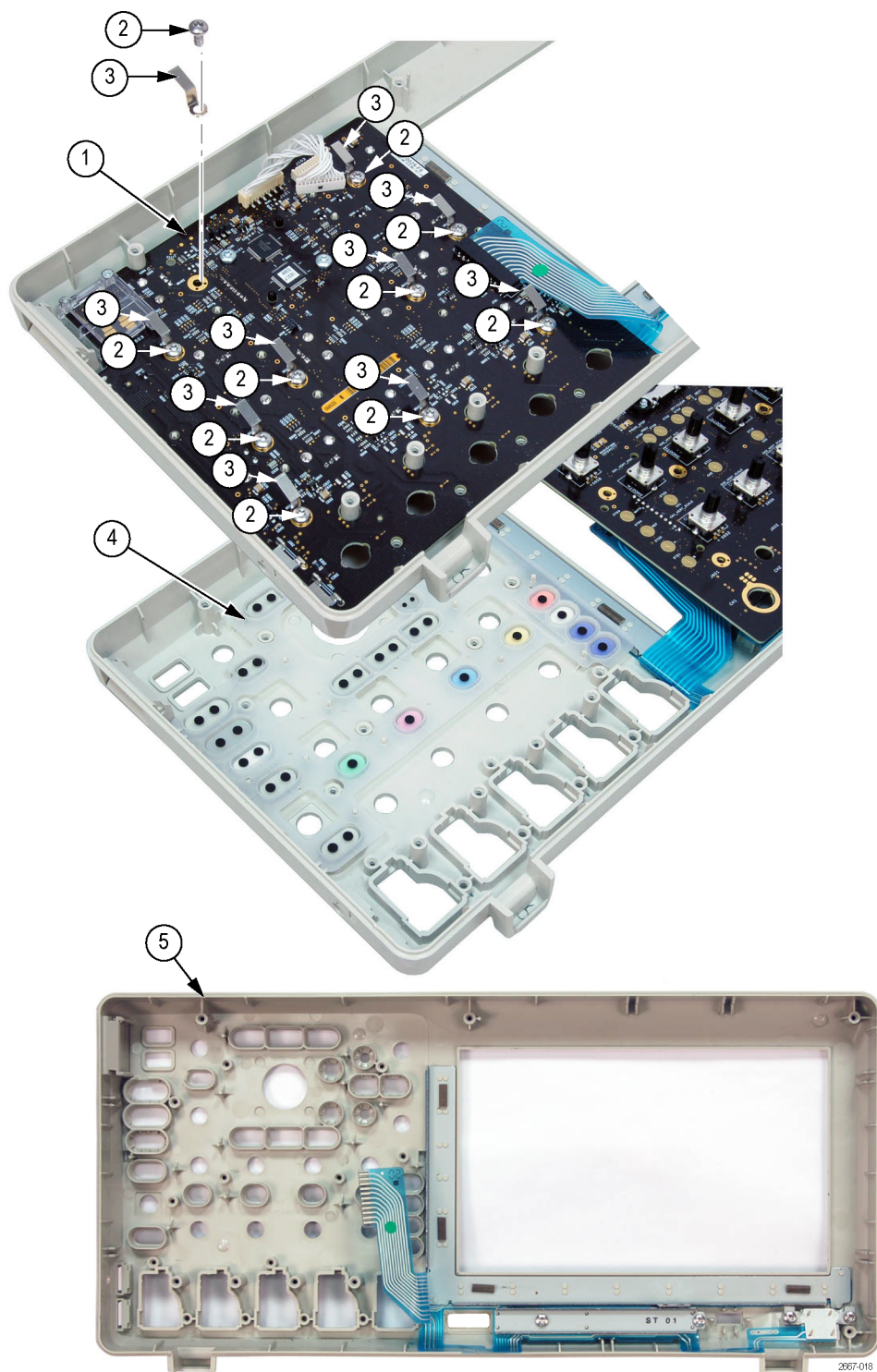
Figure 18: Exploded view: front panel board and front case
