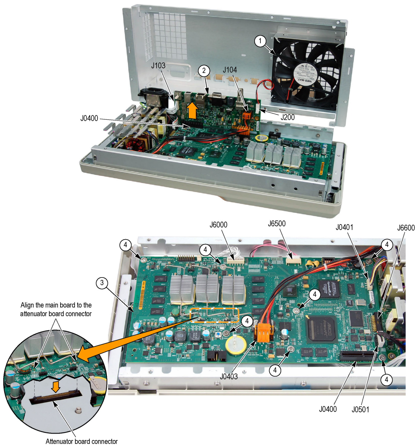
Figure 13: Exploded view: I/O and main boards
