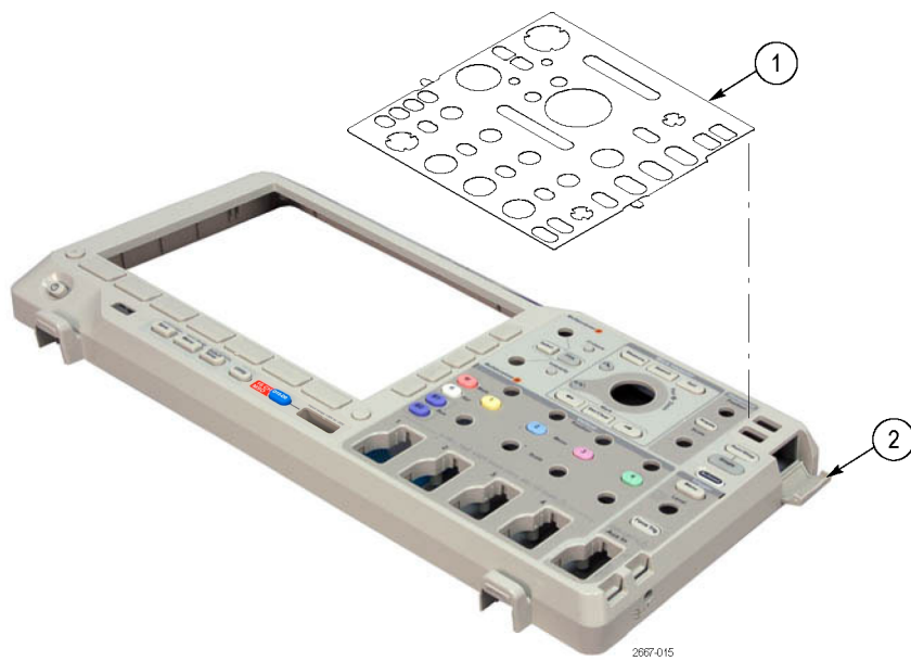
Figure 15: Exploded view: Front panel labels
