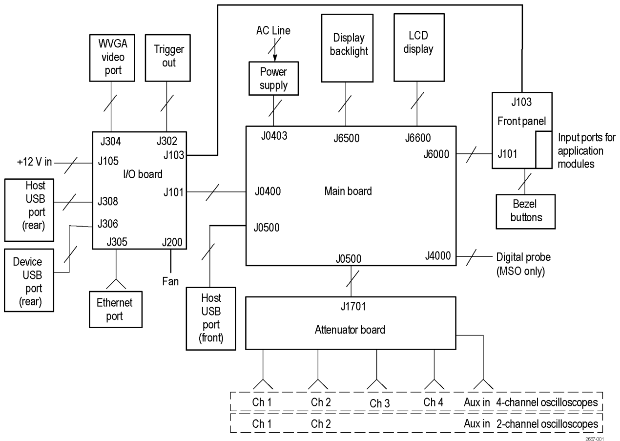
Figure 1: Oscilloscope module interconnections
