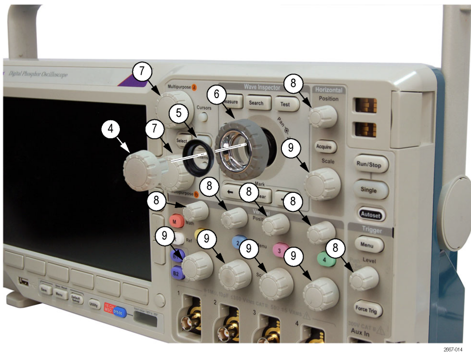
Figure 14: Exploded view: Front panel and power supply
