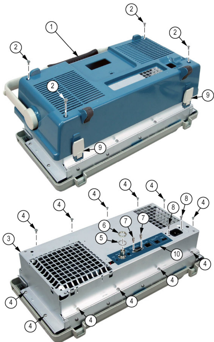
Figure 12: Exploded view: rear case and rear chassis
