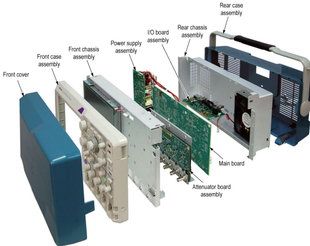
Figure 7: Locator for internal modules
