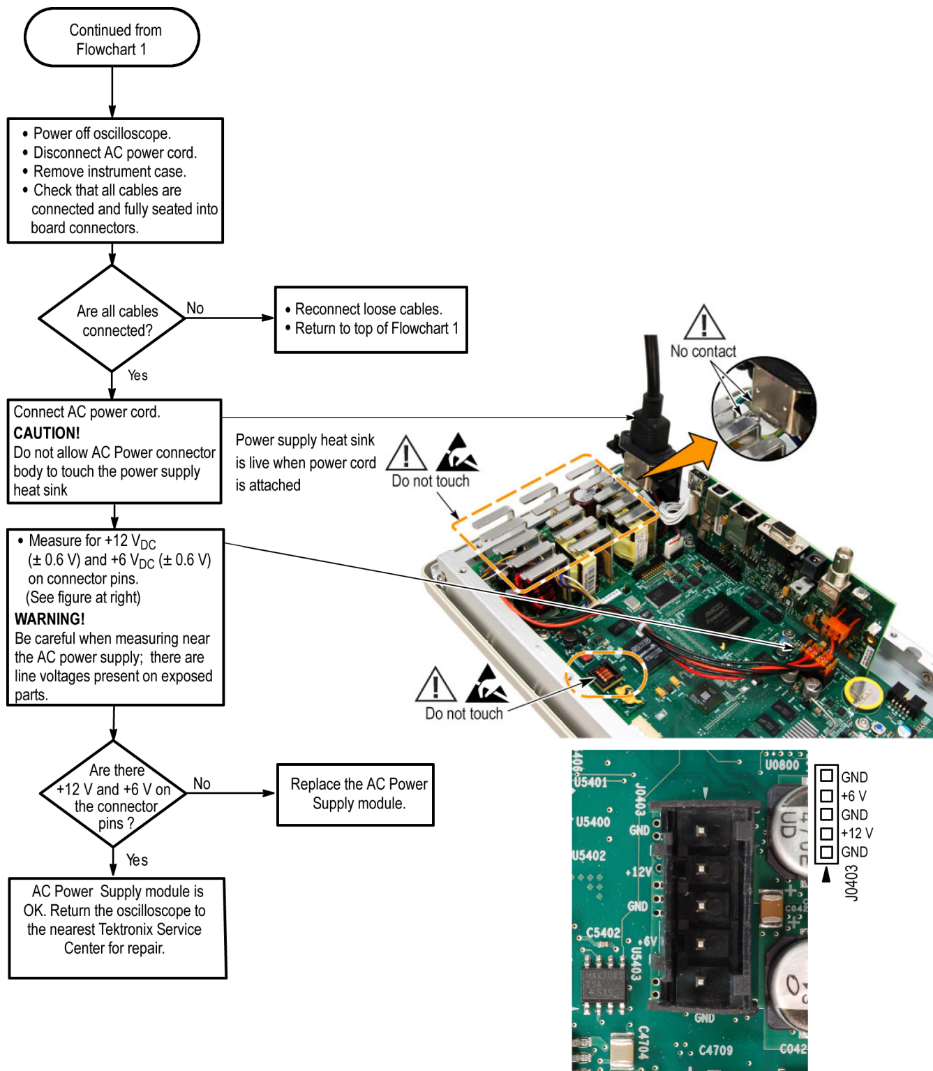
Flowchart 2 — AC power supply troubleshooting procedure
