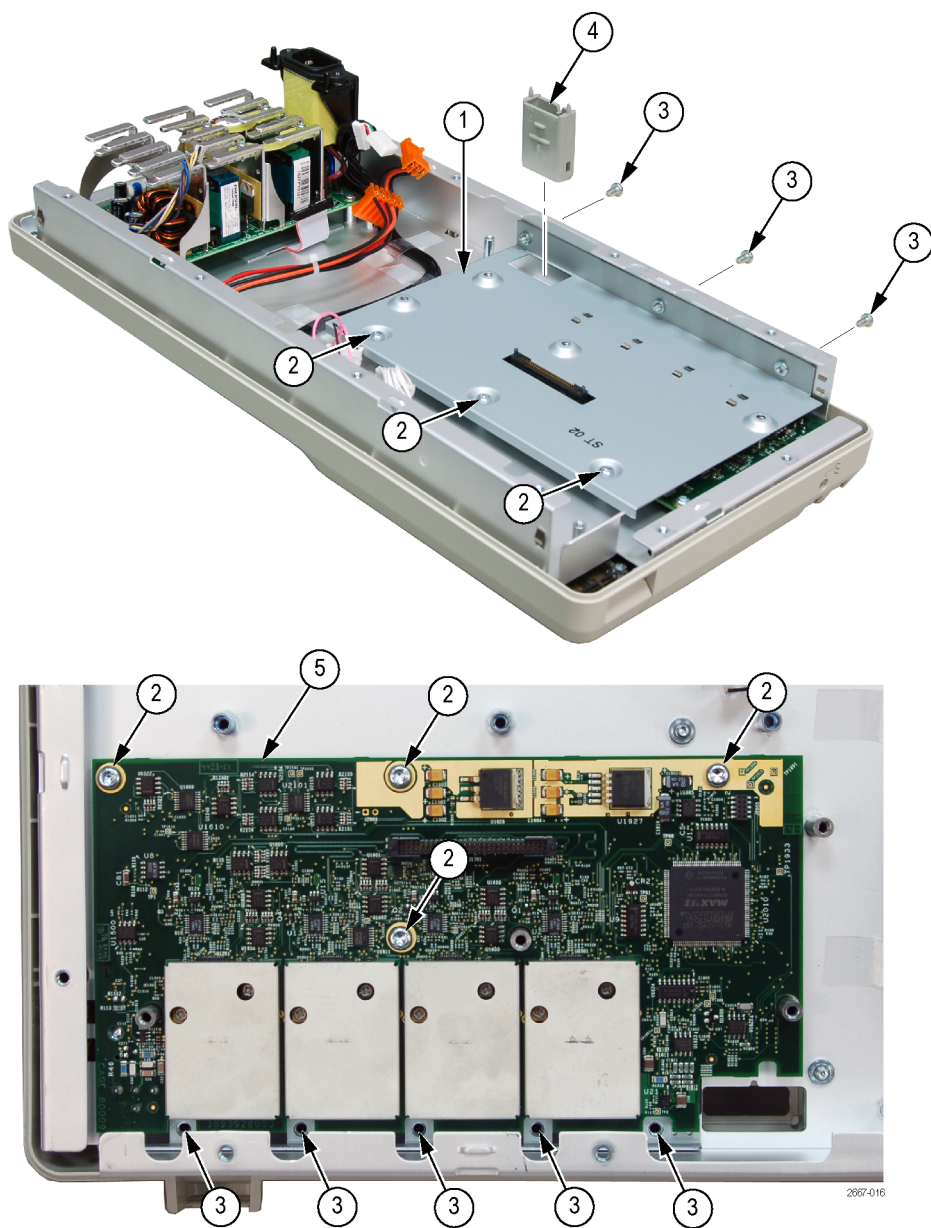
Figure 16: Exploded view: Main board shield and attenuator board
