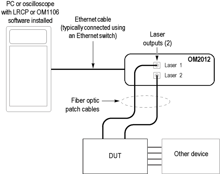
Figure 1: OM2012 connection diagram
