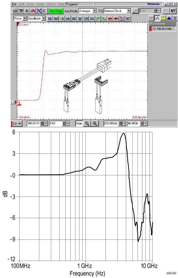
Typical rise time and frequency plots
