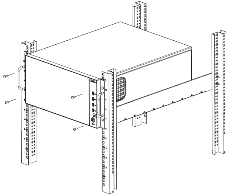
Figure 3: Assembled 4200-RM
