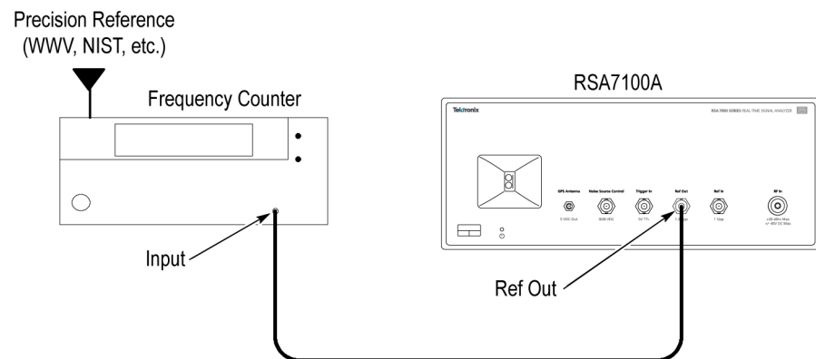
Figure 1: Connections for Reference Frequency Output Accuracy check
