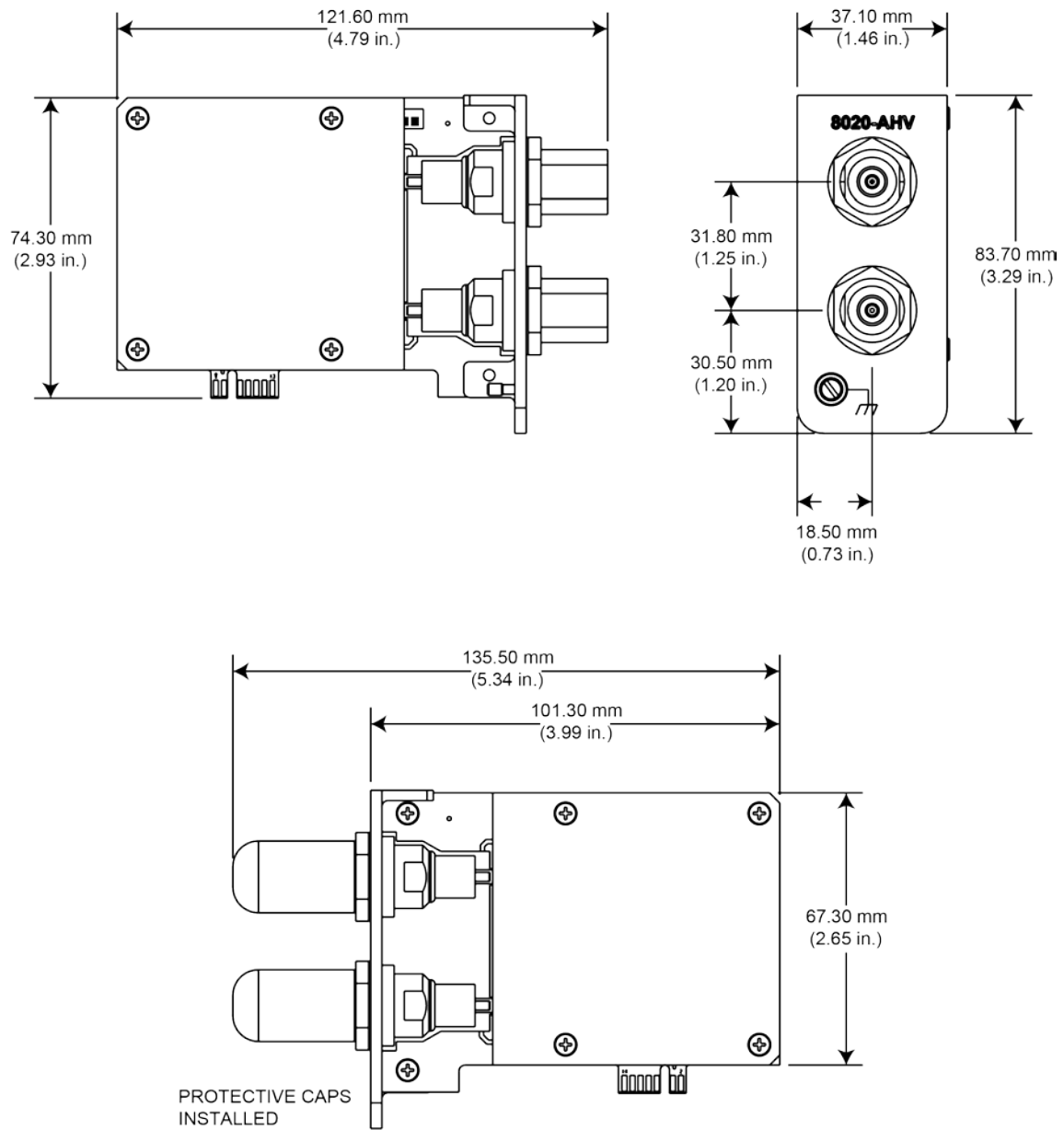
Figure 5: Model 8020-AHV dimensions
