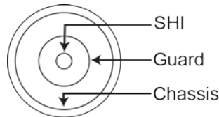
Figure 3: Connector conductors when installed in the HV and 2600/4200 channel of the Model 8020
