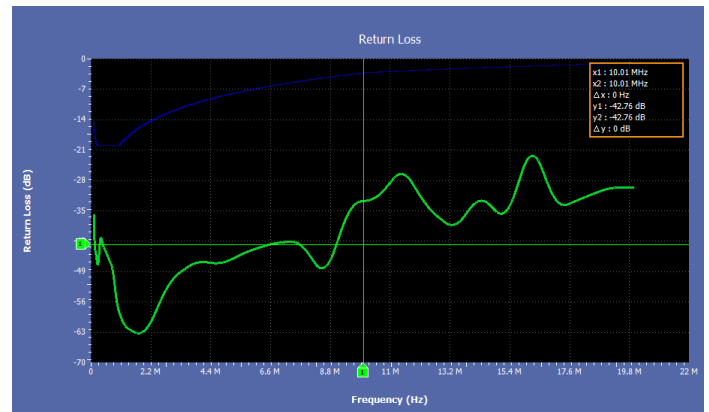
Return loss plot generated using the oscilloscope and AFG
