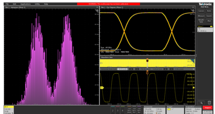
Jitter measurement
