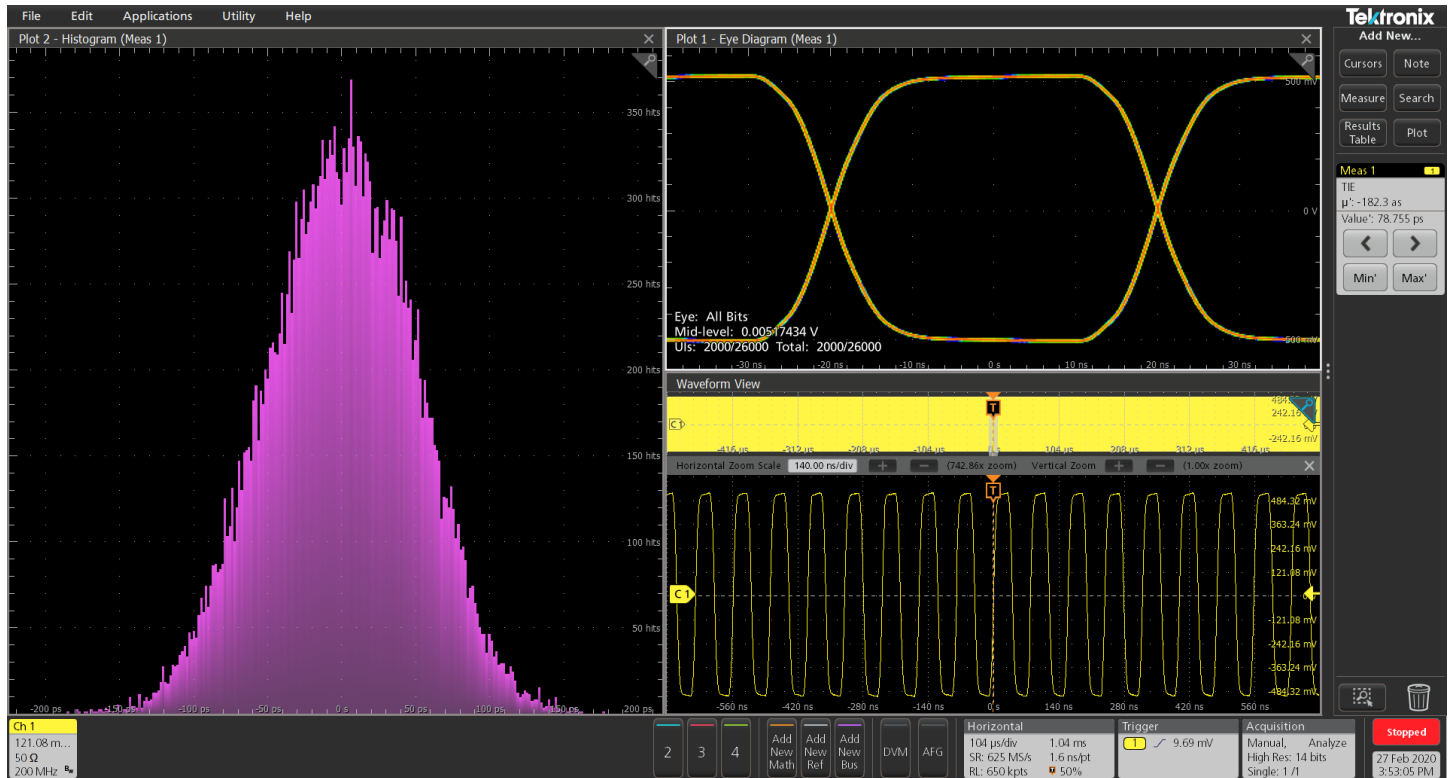
Jitter measurement
