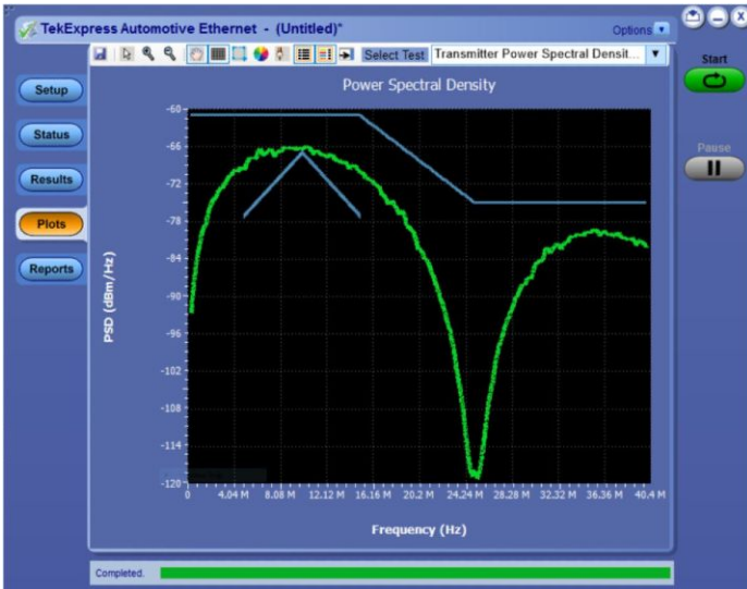
Power spectral density measurement
