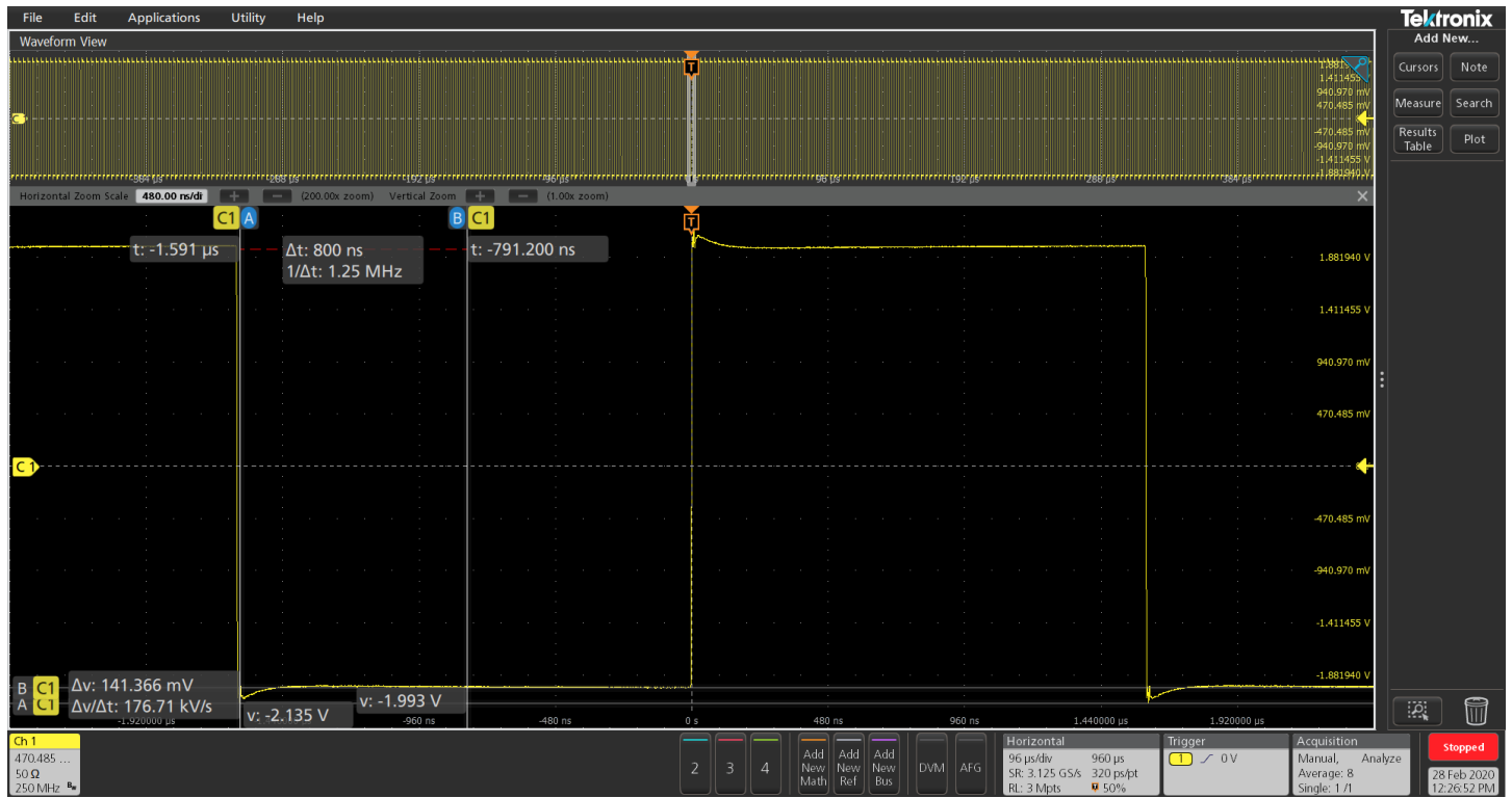
Droop measurement
