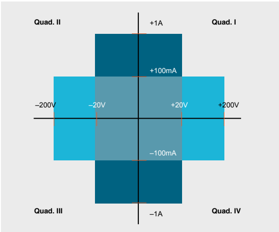
2450 power envelope.
