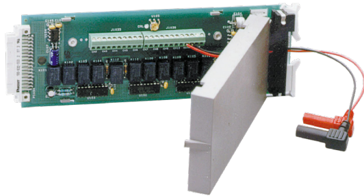
2000-SCAN 10-Channel Multiplexer.
