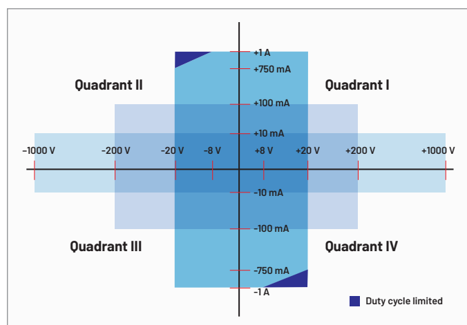
2470 power envelope.
