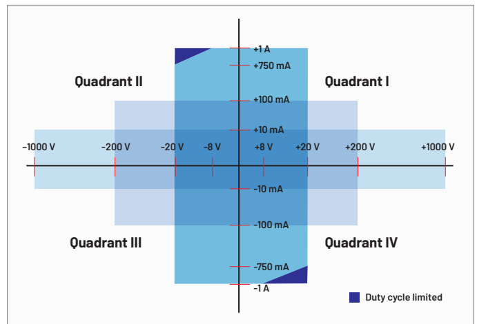
2470 power envelope.
