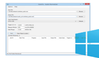
Windows Application
