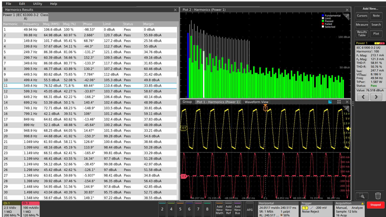
Harmonics bar graph, harmonics results table, and traverse capability via the results bar (upper right)
