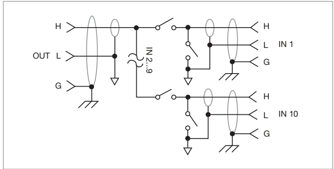
6522 schematic.
