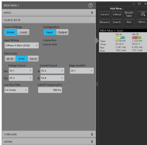
Ripple analysis configuration can be set to look into line and switching ripple
