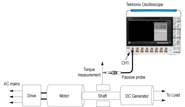
Torque measurement setup using the torque sensor method
