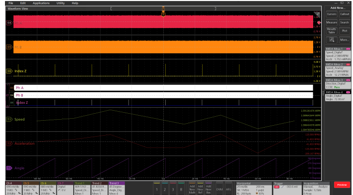
Measuring motor speed and direction using QEI method. The QEI signals (Phase A, B, and Z index) are shown for reference by connecting both Analog (TPP1000) and Digital (TLP058) probes.
