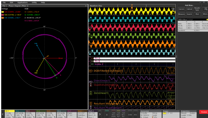
DQ0 measurement running on the 5 Series MSO. They are represented on the phasor diagram as Q (green), D (orange), and Z (white) vectors and their scalar values are available in the results badge on the right. The DQ0 waveforms are shown as Math M1, Direct (purple), Quadrature (red), and Zero (green).
