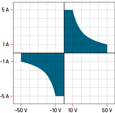
Figure 16: MPSU50-2ST Power Envelope
