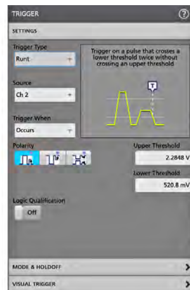
Figure 7: Configuration menus are accessed by simply double-tapping on the item of interest on the display. In this case, the Trigger badge was double-tapped to open the Trigger configuration menu.
