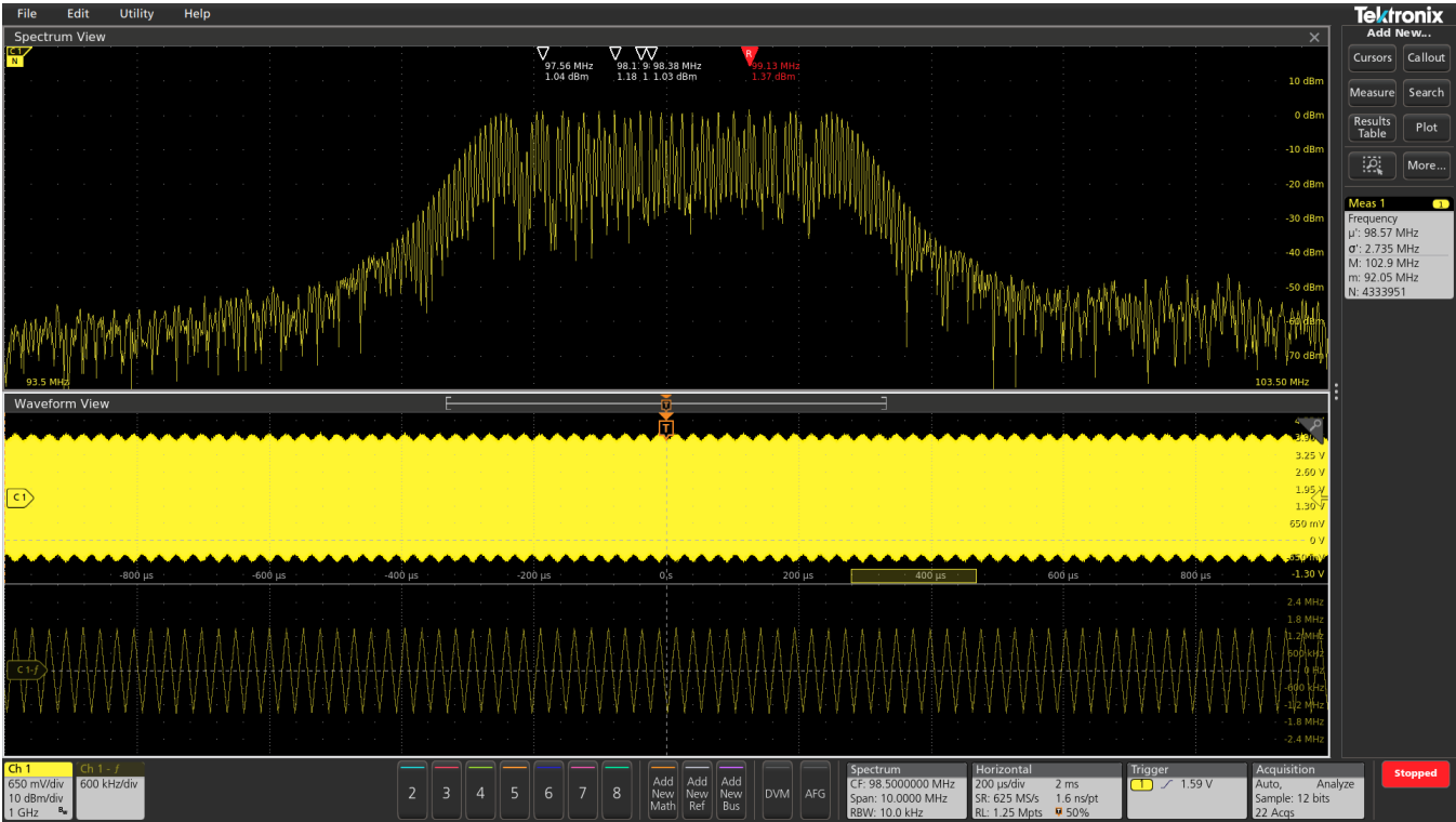
The lower trace is the frequency vs. time trace derived from the input signal. Notice that the Spectrum Time is positioned during a transition from the lowest frequency to the middle frequency, so the energy is spread across a number of frequencies. With the frequency vs. time trace, you can easily see the different frequency hops, simplifying characterization of how the device switches between frequencies.
