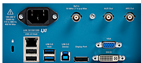
The I/O you need to connect the 5 Series MSO to the rest of your design environment.
