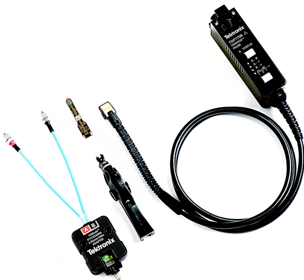
Figure 18: TDP7700 Series probe with a selection of available tips
