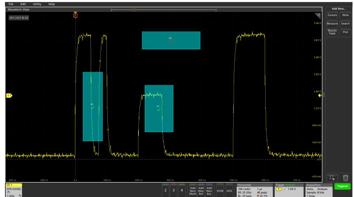
Figure 16: Boolean logic trigger qualification. Boolean logic using logical OR allows triggering on a specific anomaly in the signal.
