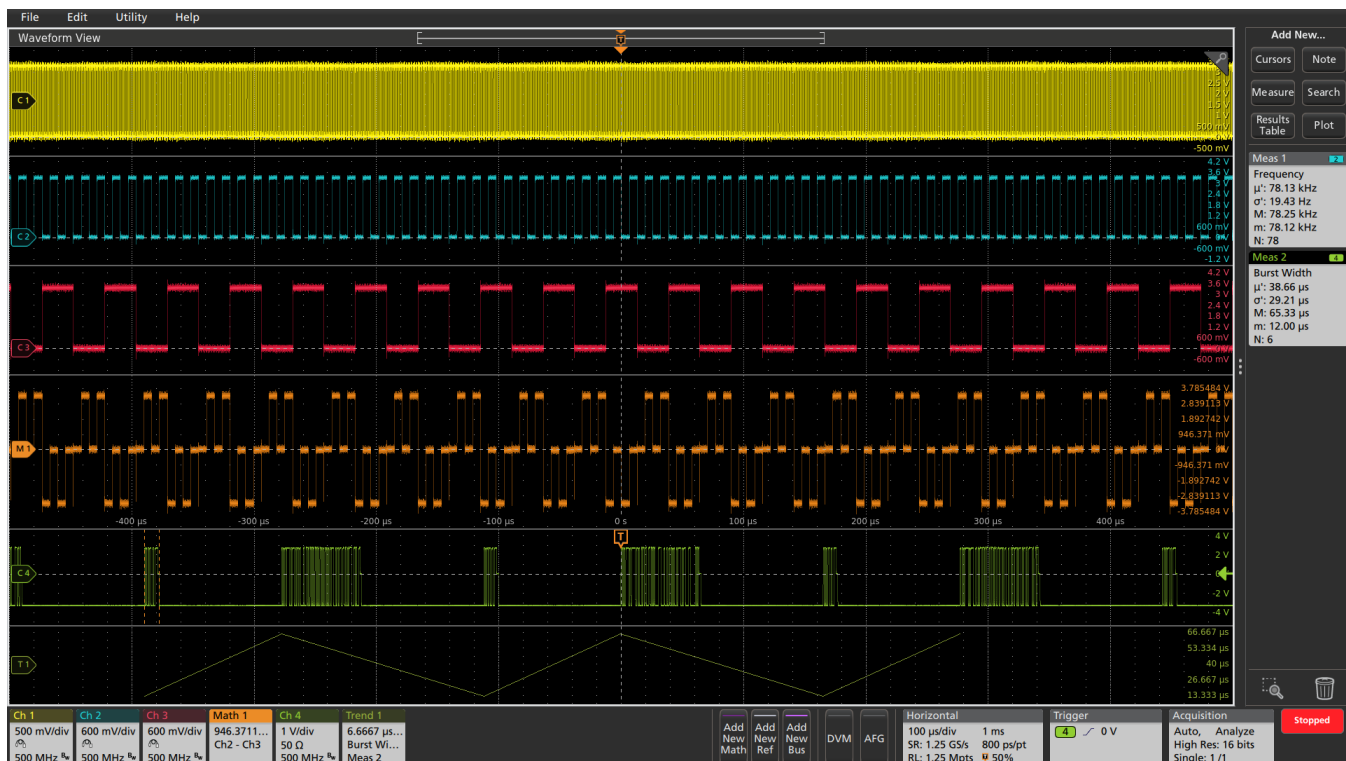
Figure 20: Using measurements to characterize burst width and Frequency.
