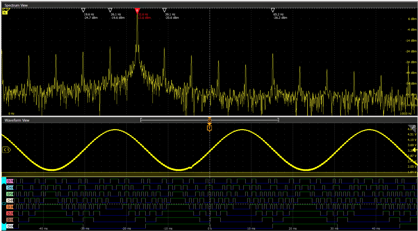
Figure 4: Beyond just analog and digital, FlexChannel inputs include Spectrum View. This Tektronix-patented technology enables you to simultaneously view both analog and spectral views of all your analog signals, with independent controls in each domain. For the first time ever, oscilloscope-based frequency-domain analysis is as easy as using a spectrum analyzer while retaining the ability to correlate frequency-domain activity with other time-domain phenomena.
