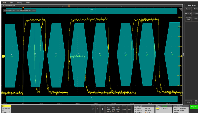
Figure 14: Visual Trigger areas isolate an event of interest, saving time by only capturing the events you want to see.
