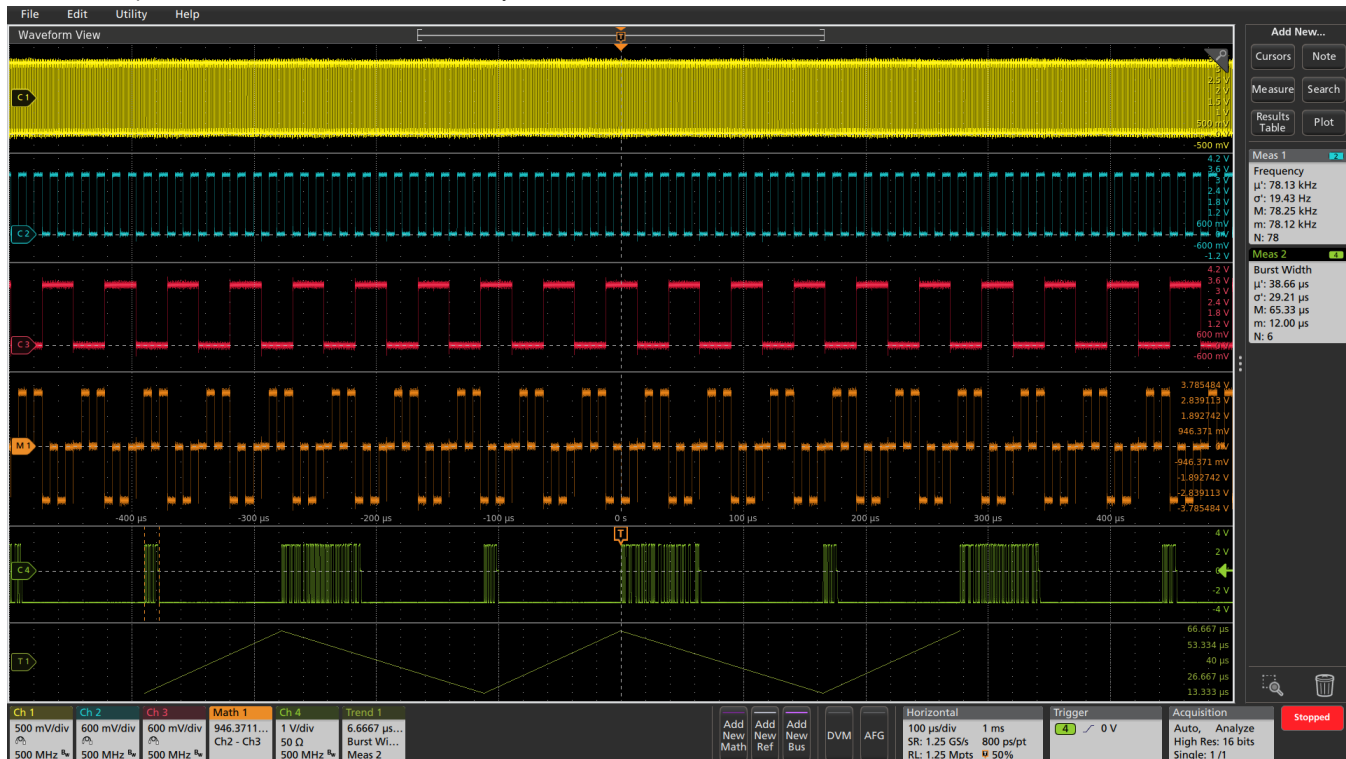
Figure 5: Stacked display mode enables easy visibility of all waveforms while maintaining maximum ADC resolution on each input for the most accurate measurements.
