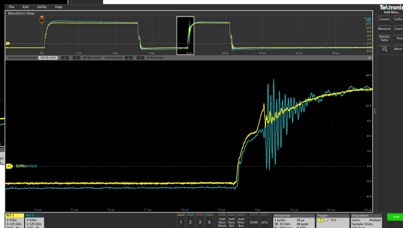
V GS Turn-on
