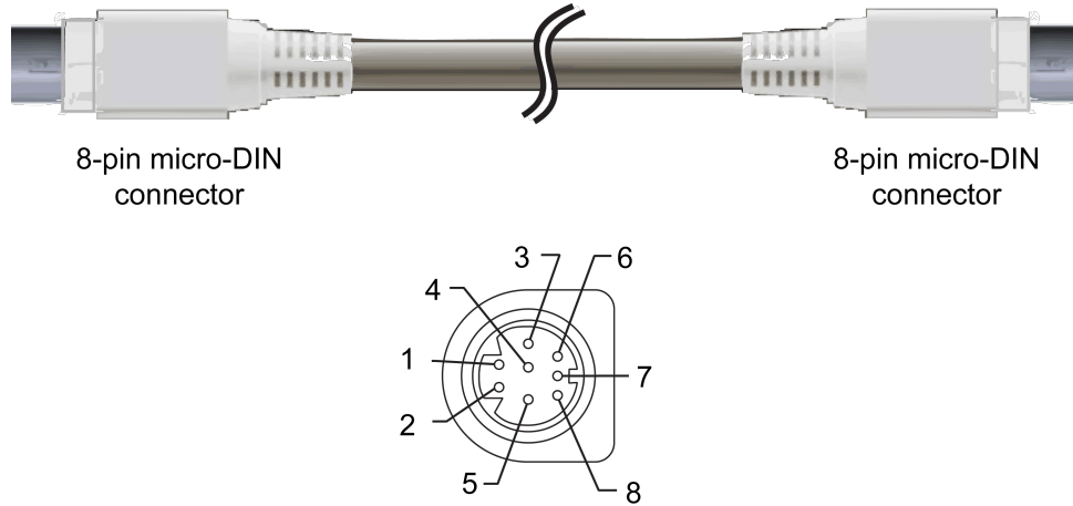
Figure 2: Model 8501 pinouts
