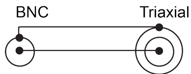
Figure 2: Model 237-BNC-TRX Schematic
