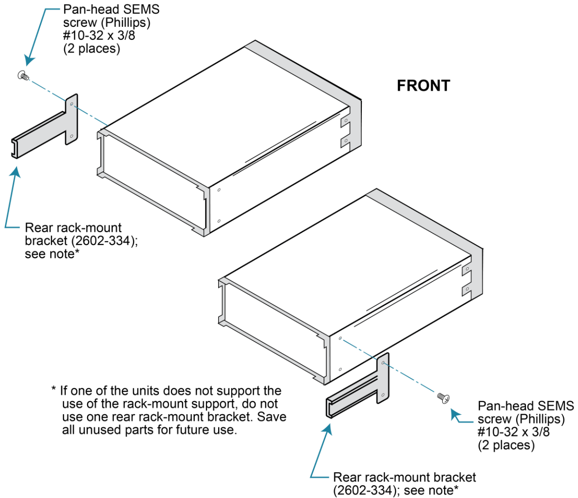
Figure 2: Rear rack-mount bracket
