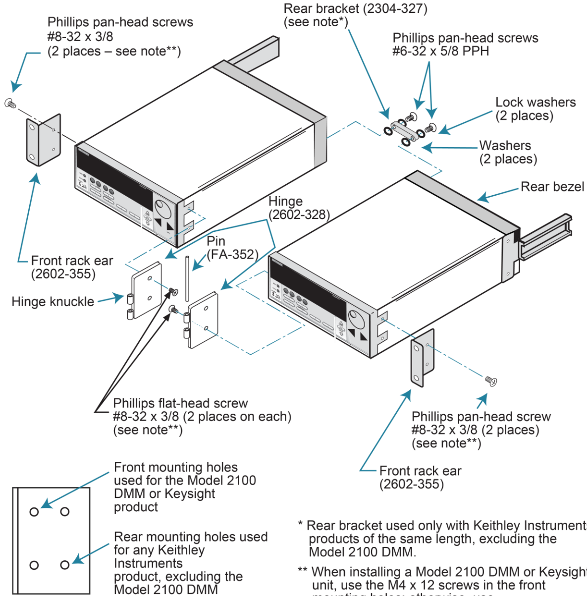
Figure 3: Secure the instruments to each other
