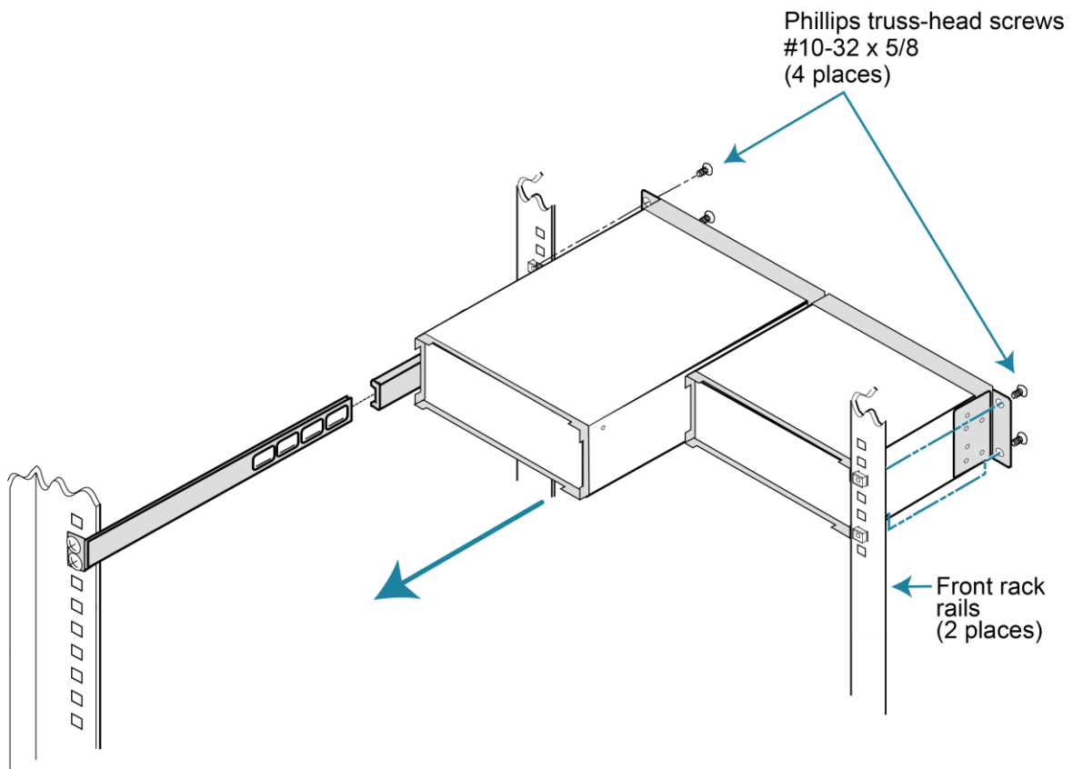
Figure 6: Securing different length track rails
