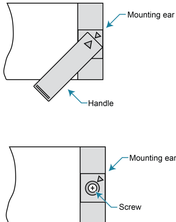
Figure 1: Handle removal
