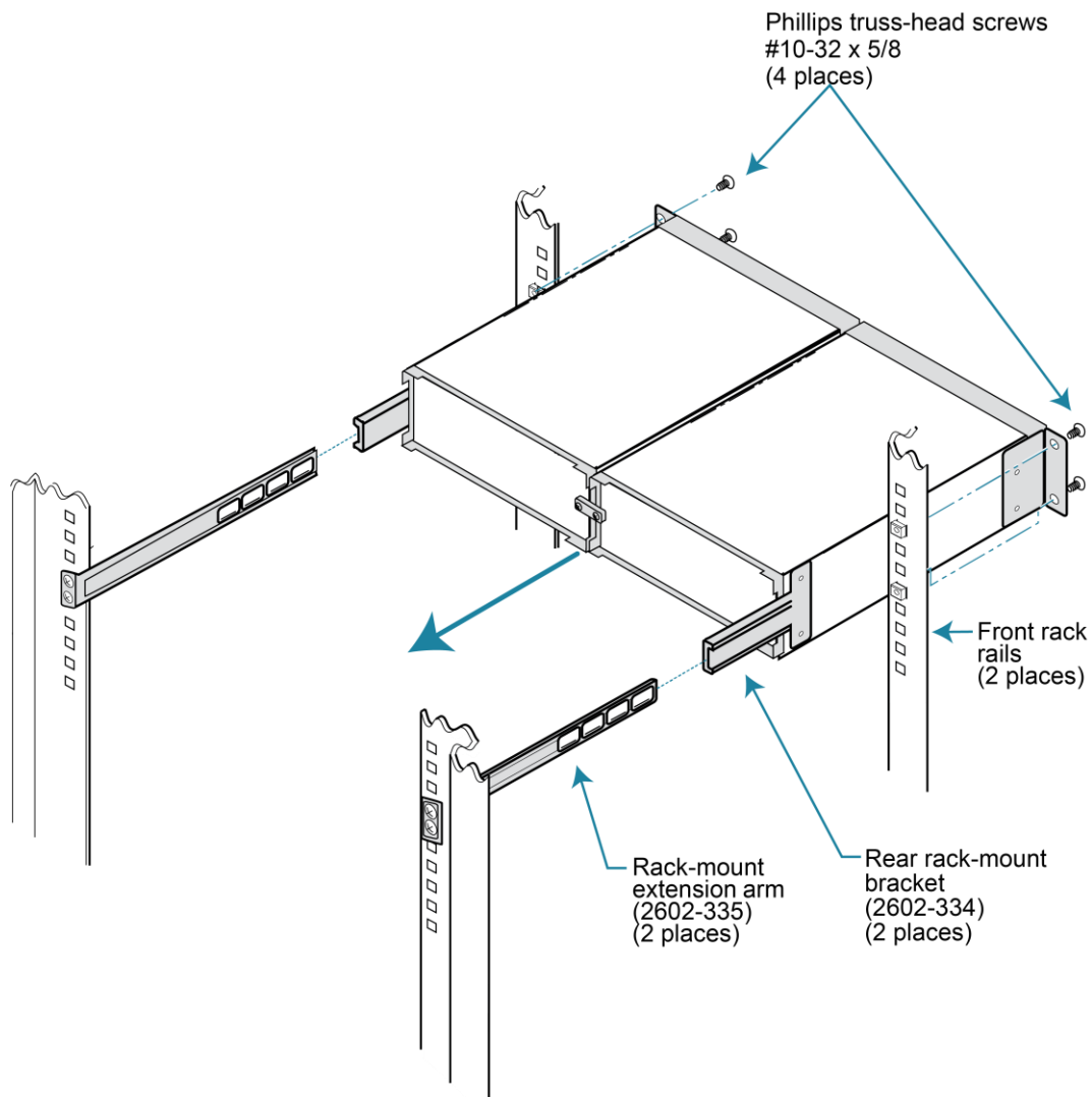
Figure 5: Install the instruments
