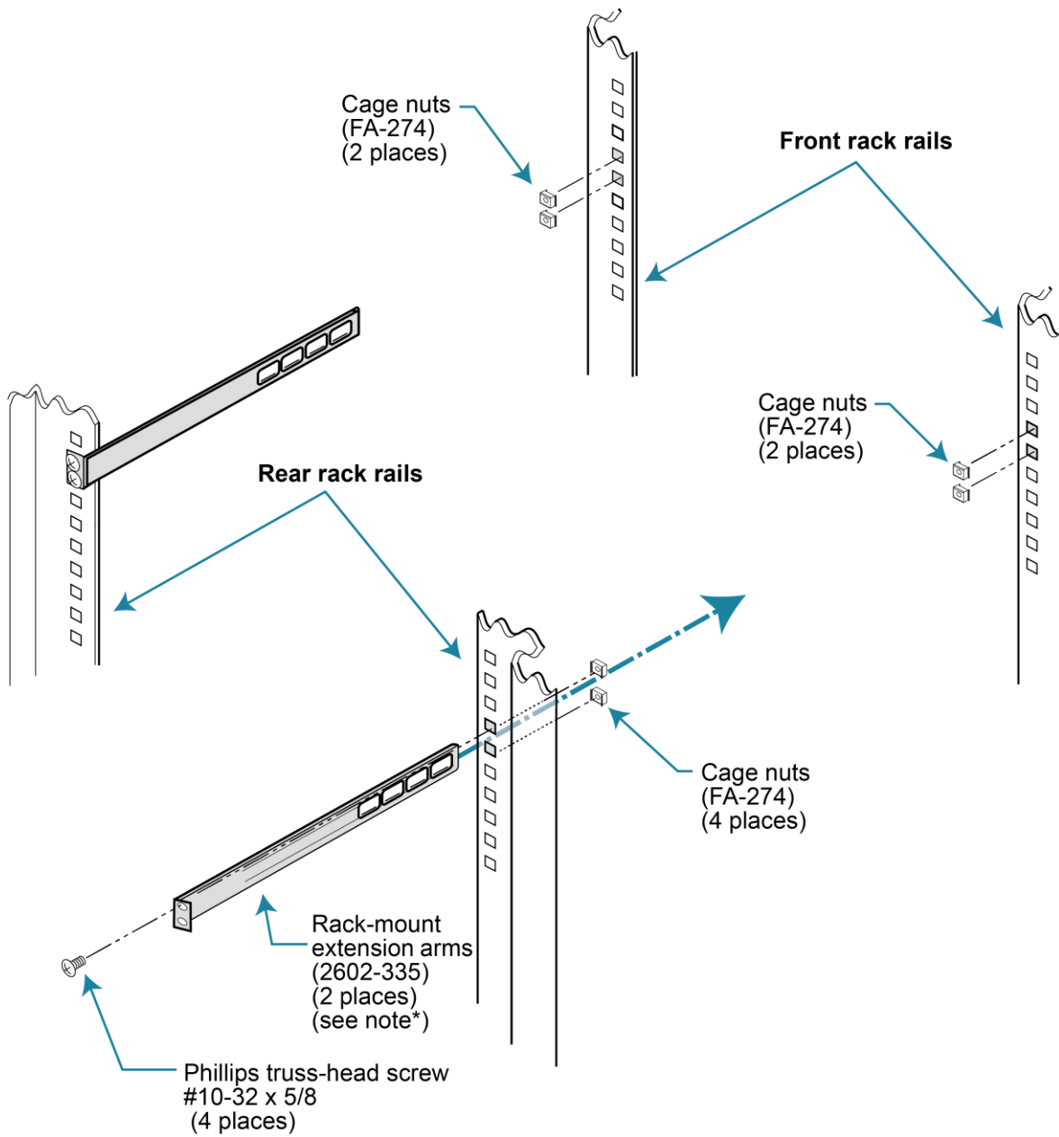
Figure 4: Rack-mount extension arms
