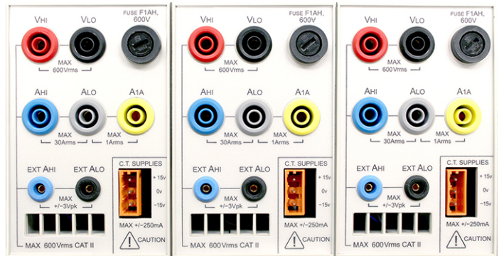
PA4000 Rear Panel - Input Modules on a 3-channel instrument
