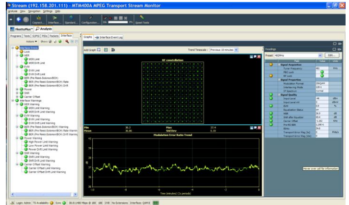
RF Trending QAM interface (with dual alarming)
