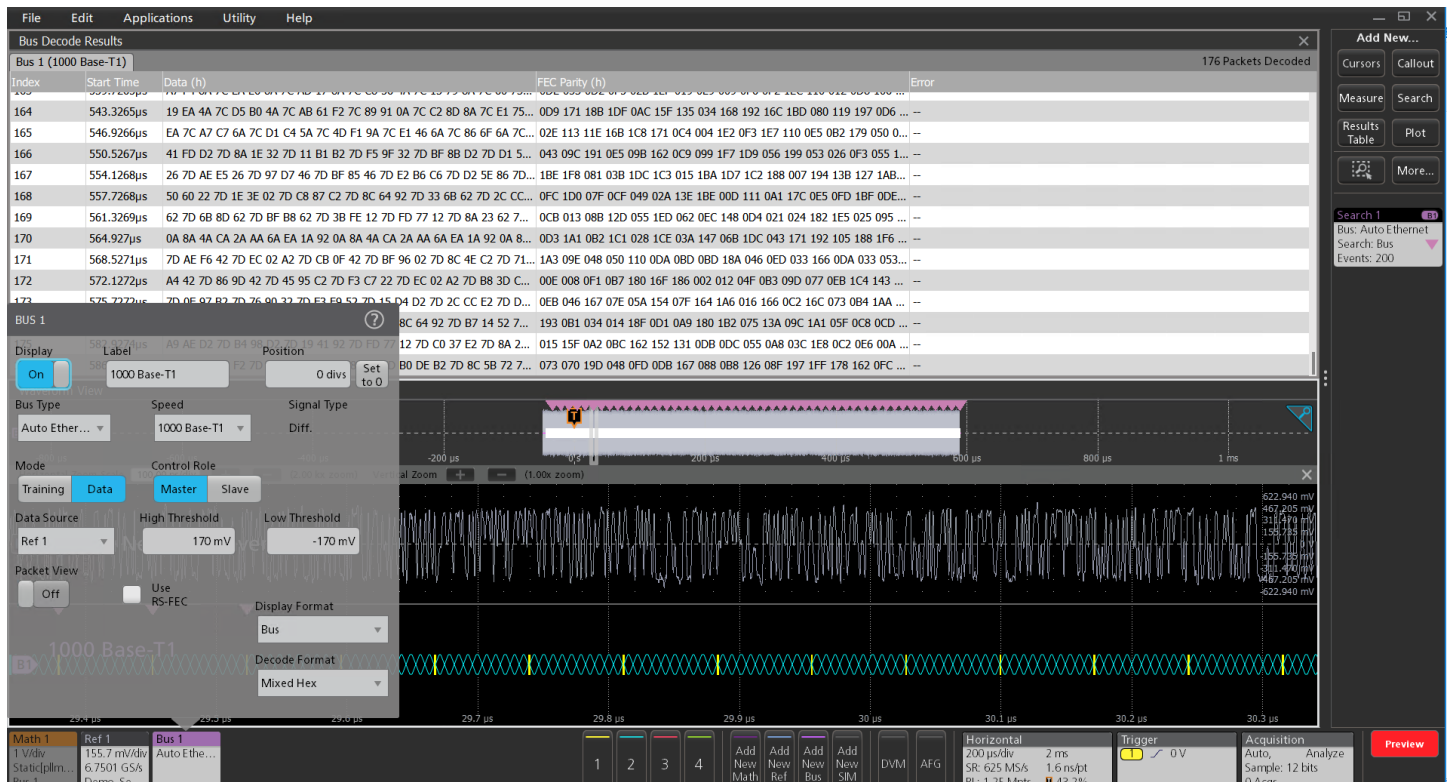
1000baseT1 bus showing decode with packet view off and RS-FEC off. Control header was searched with 200 occurrences
