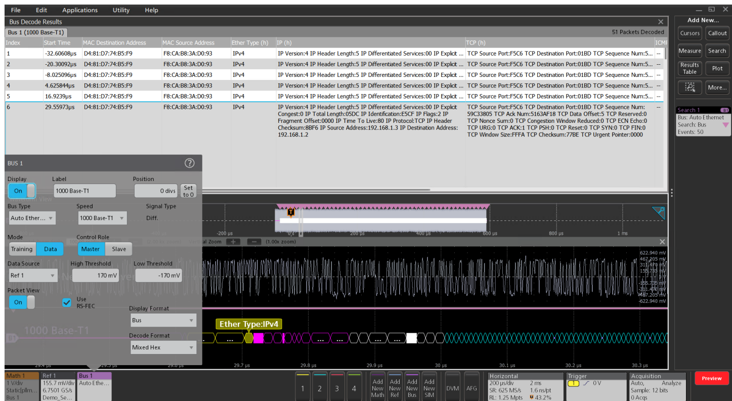
1000baseT1 bus showing decode with packet view on and RS-FEC on. EtherType IPV4 TCP type was searched with 50 occurrences
