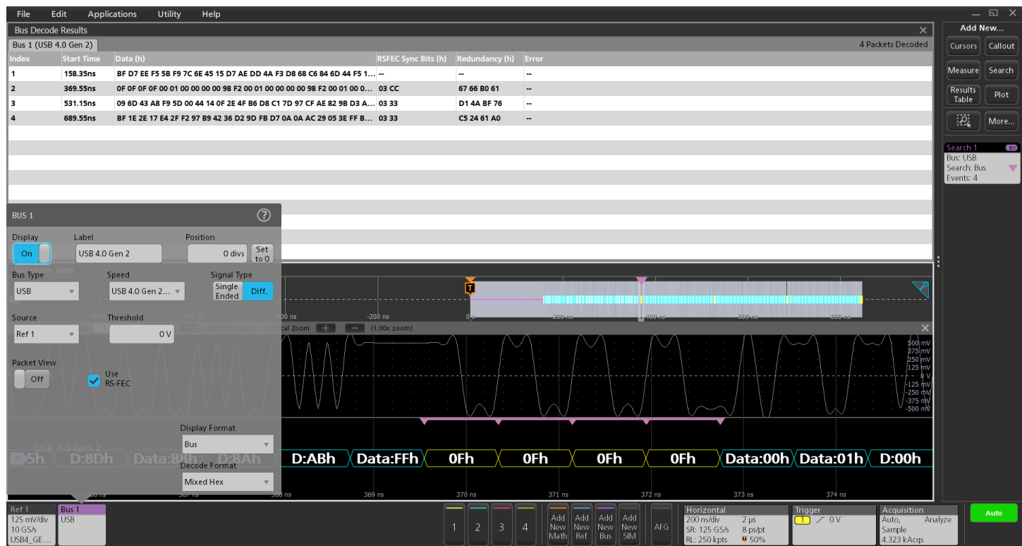
USB4 Gen2 bus setup showing decode with packet view Off with RSFEC. START_RSFEC searched with 4 occurrences.
