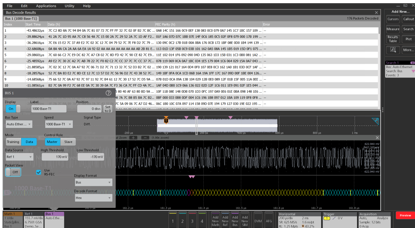
1000baseT1 bus showing decode with packet view Off and RS-FEC on. RS-FEC error type was searched with 3 occurrences
