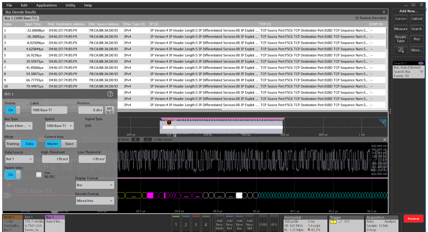
1000baseT1 bus showing decode with packet view on and RS-FEC off
