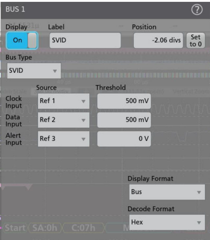
Bus configuration
