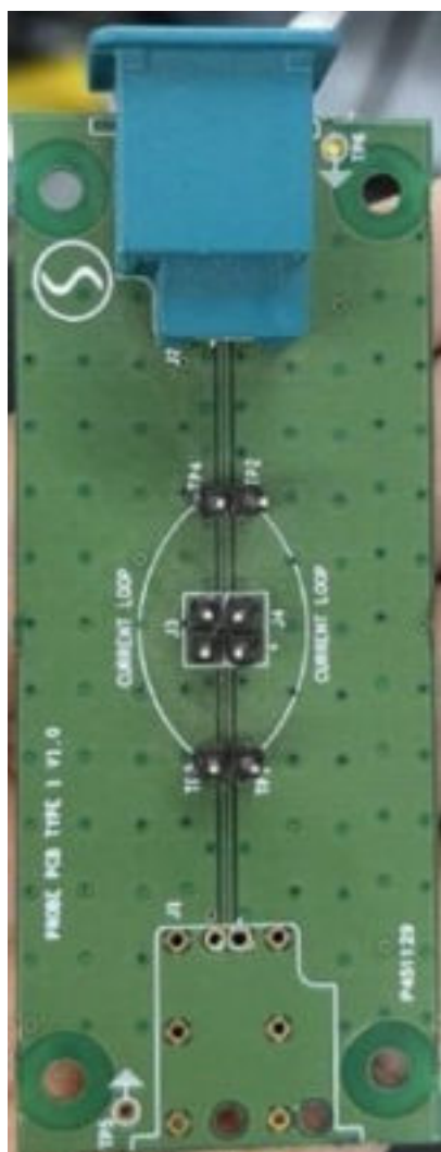
PROBE PCB TYPE 1
