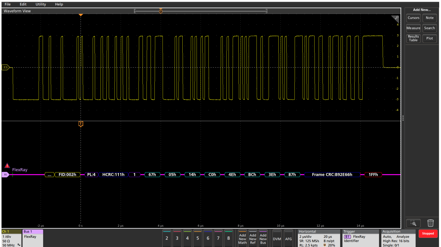
Decoded FlexRay bus, with the acquisition triggered on a specified identifier value.
