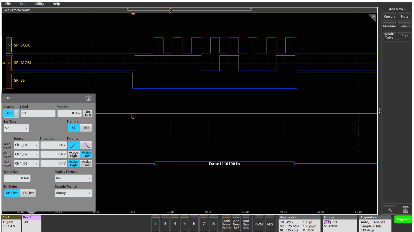
SPI bus, captured with digital channels, showing binary display format of the color-coded SPI bus decoding.
