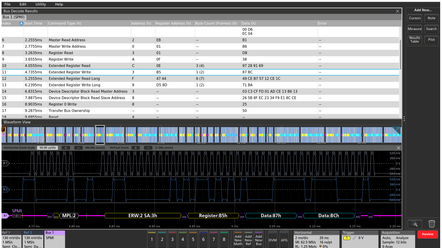
Protocol Decode Results Table provides a time-stamped, tabular view of all captured packets on the SPMI bus.
