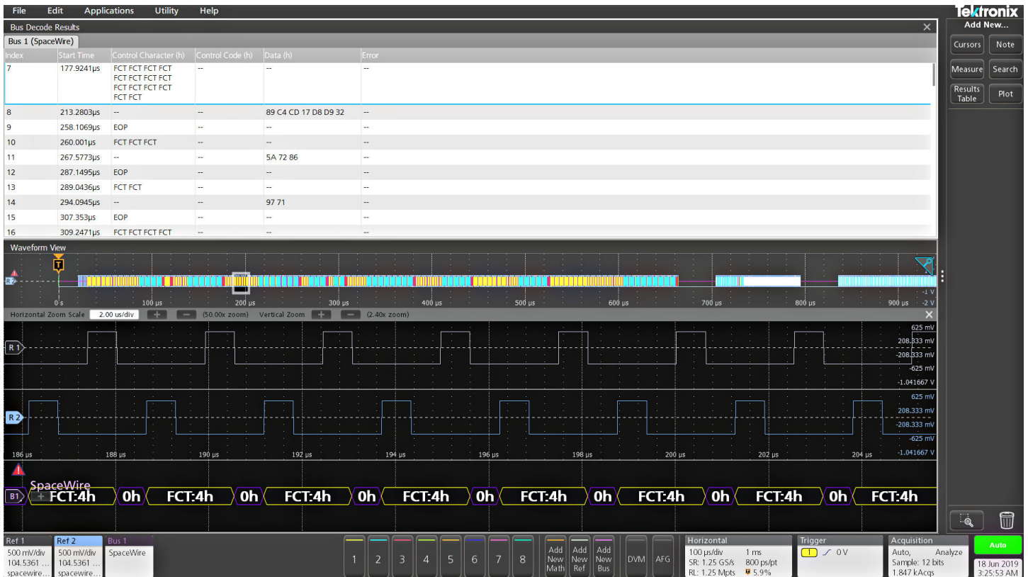
The Protocol Decode Results Table provides a time-stamped, tabular view of all captured packets on the SpaceWire bus.
