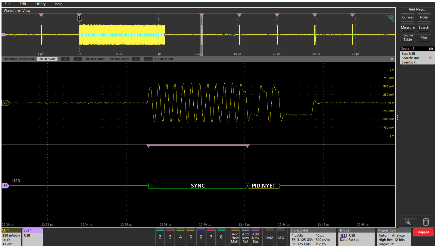
Triggering on a specific data pattern on the USB 2.0 bus and automatically searching on Sync.
