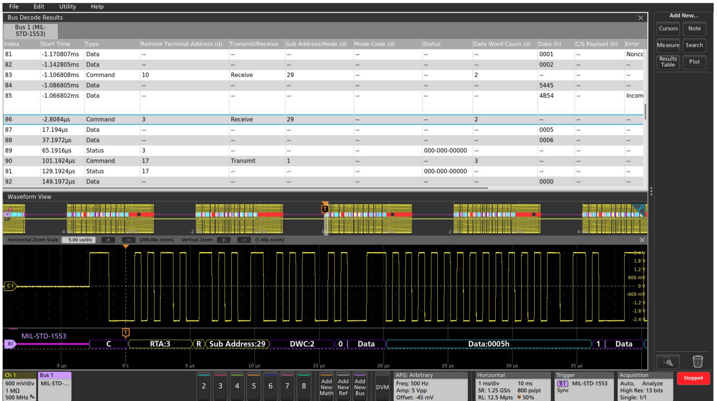
Protocol Decode Results Table provides a time-stamped, tabular view of all captured MIL-STD-1553 packets.
