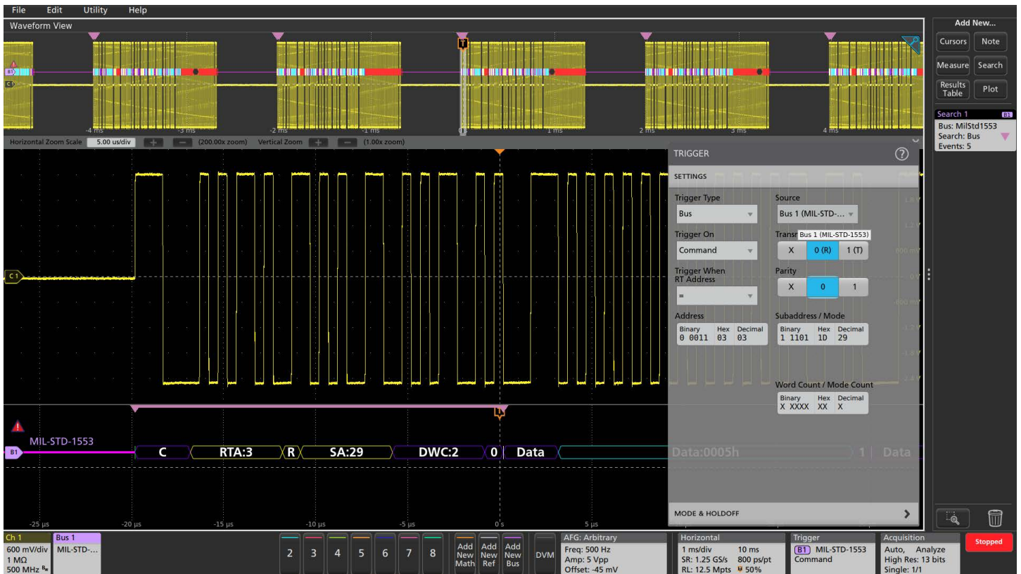
Triggering on a specific command pattern on the MIL-STD-1553 bus and automatically searching on the same pattern.
