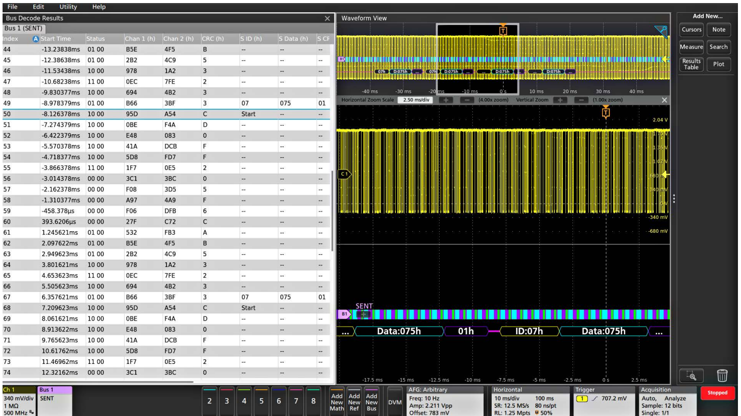
Protocol Decode Results Table provides a time-stamped, tabular view of all captured packets on the SENT bus.
