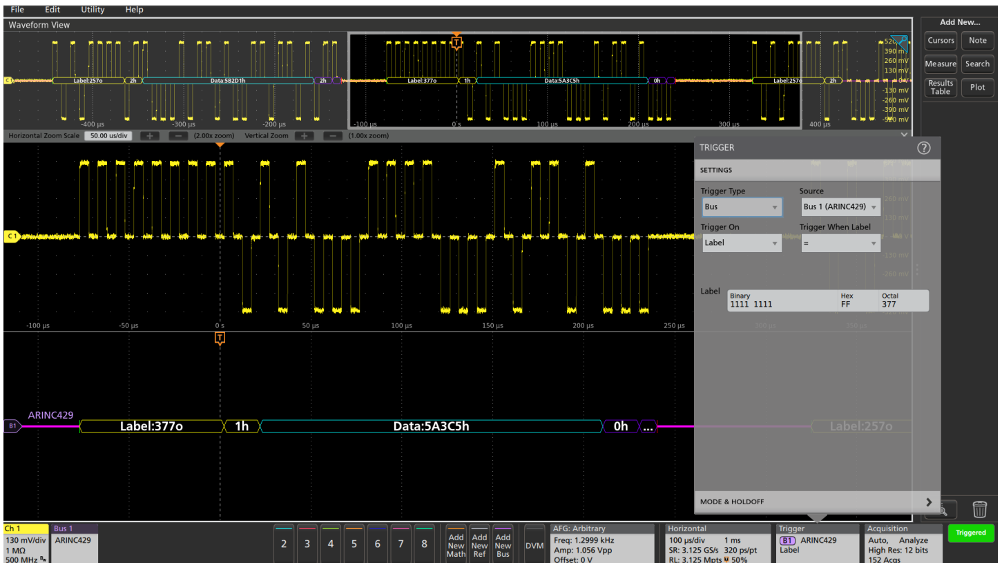
Decoded ARINC 429 bus, with the acquisition triggered on a specified label value.
