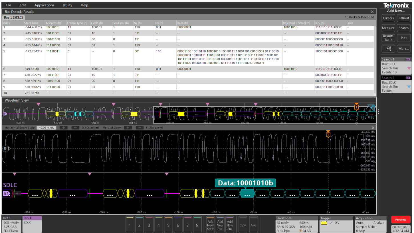
The Protocol Decode Results Table provides a time-stamped, tabular view of all captured packets on the SDLC bus.
