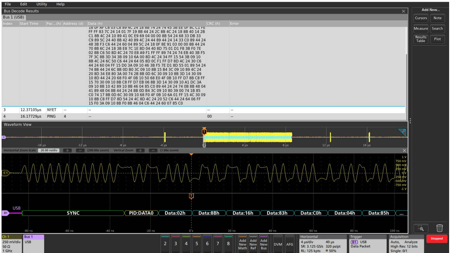
Protocol Decode Results Table provides a time-stamped, tabular view of all captured packets on the USB bus.
