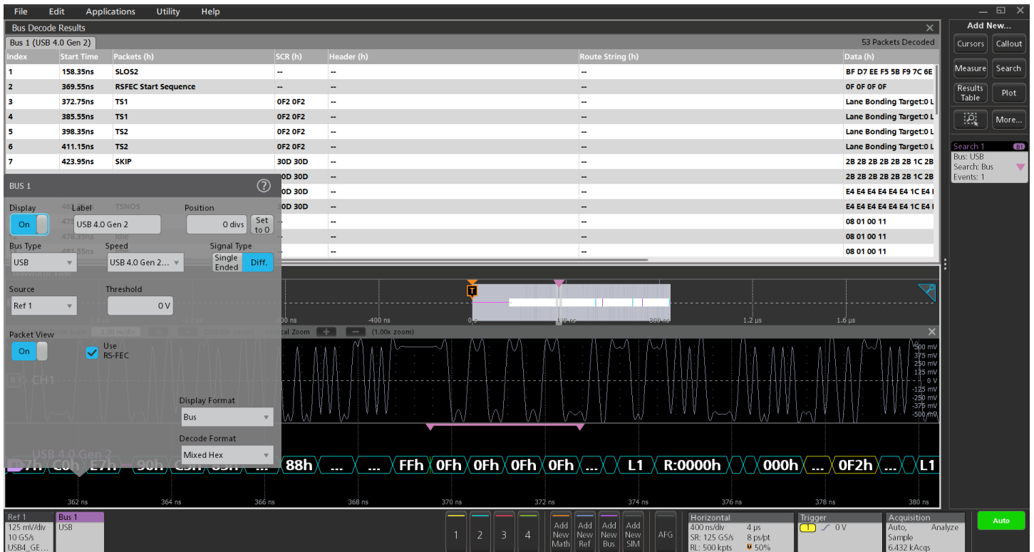
USB4 Gen2 bus setup showing decode with packet view ON with RSFEC. START_RSFECS searched with 1 occurrence.
