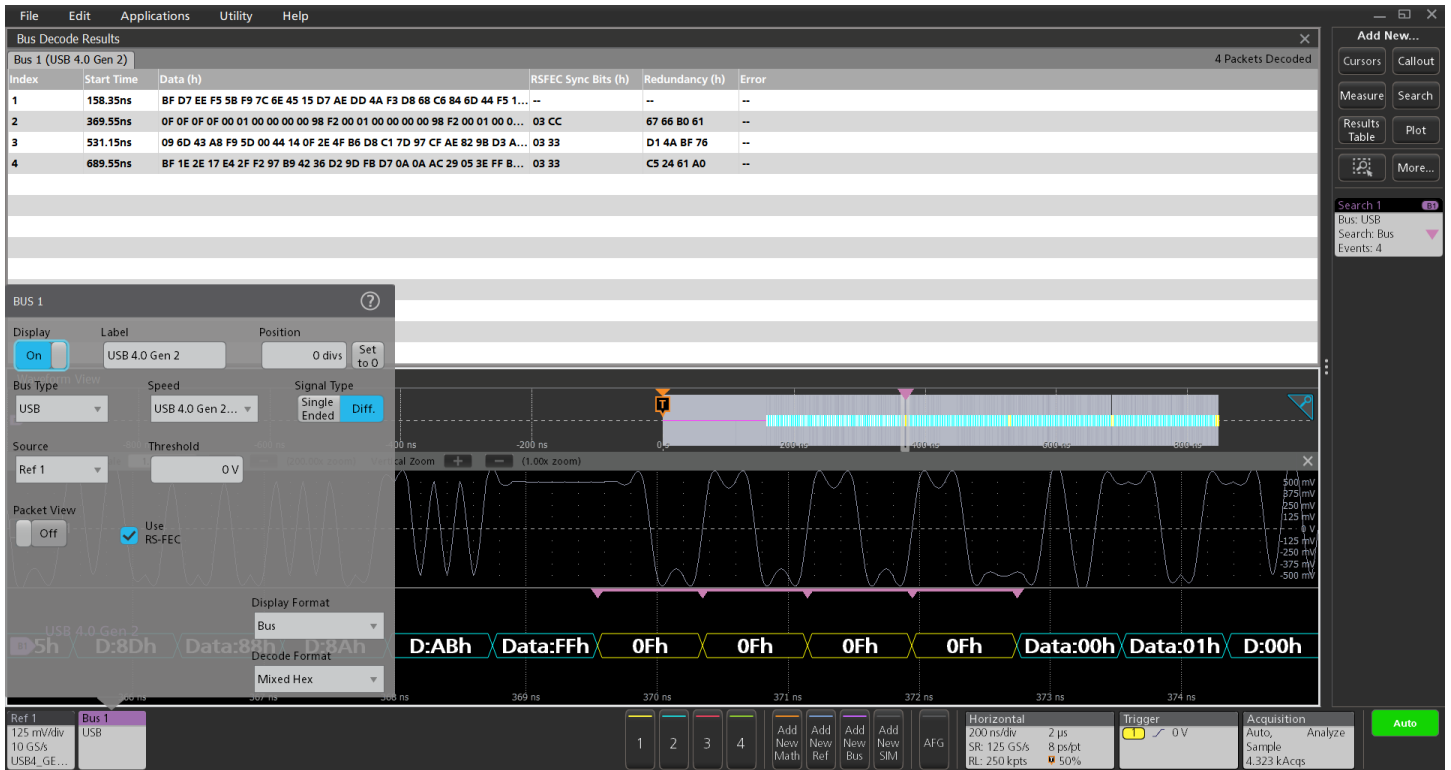
USB4 Gen2 bus setup showing decode with packet view Off with RSFEC. START_RSFECS searched with 4 occurrences.
