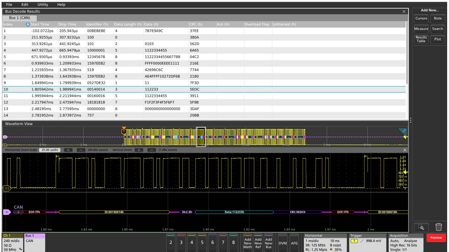
Protocol Decode Results Table provides a time-stamped, tabular view of all captured packets on the CAN bus.
