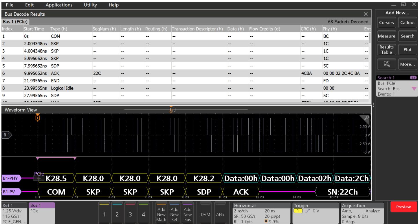
PCIe Gen 2 bus setup and MixedHex display, showing decode with packet view on. K28.5 searched with 1 occurrence.
