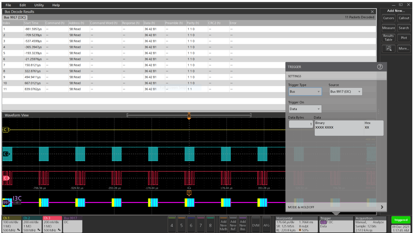
Triggering on a specific 7-Bit read address value on the I3C bus.
